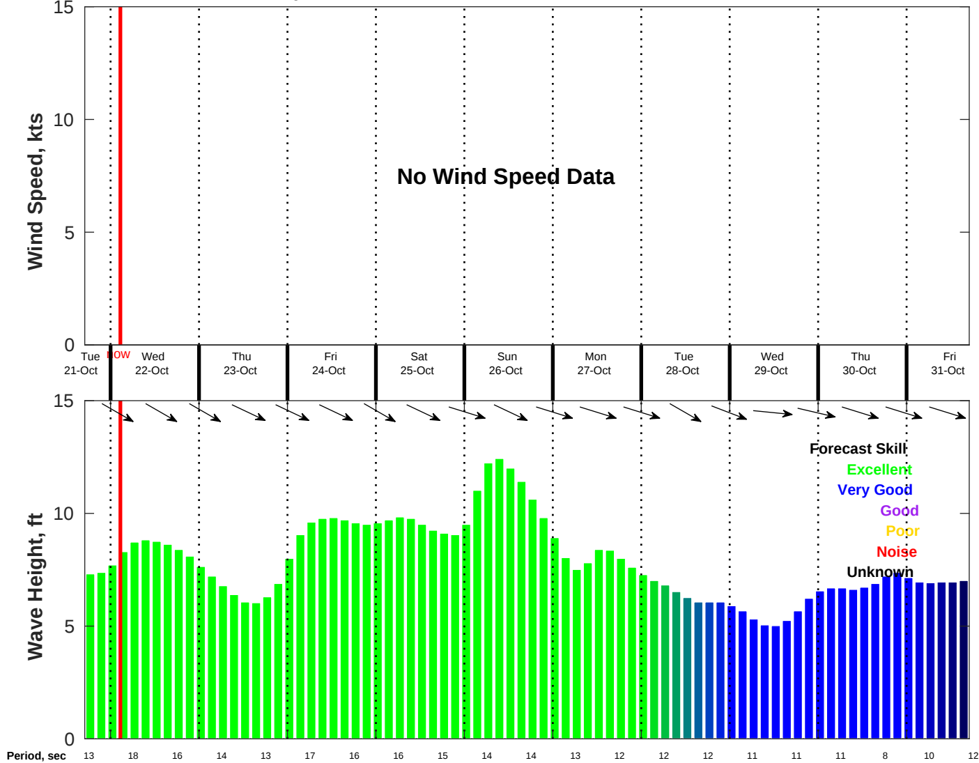
Wind & Wave Forecast for Diablo Canyon CDIP MFWAM from 21-Oct-2025 17:00:00 to 31-Oct-2025 17:00:00
