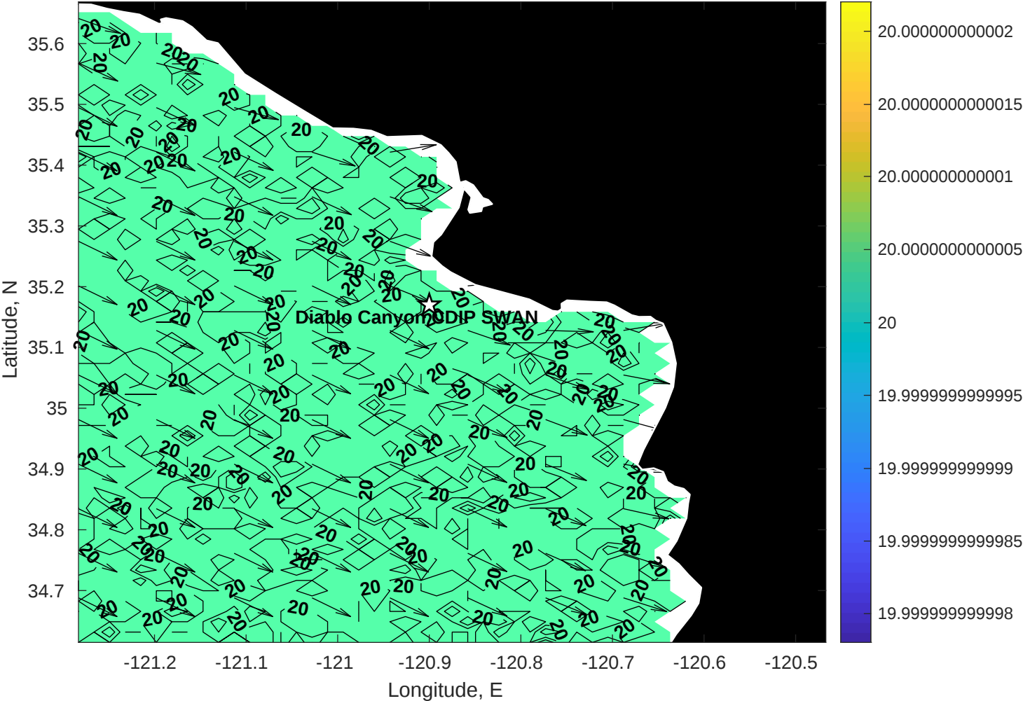
Wave Period (sec) for Diablo Canyon CDIP SWAN at 22-Oct-2025 08:00:00
