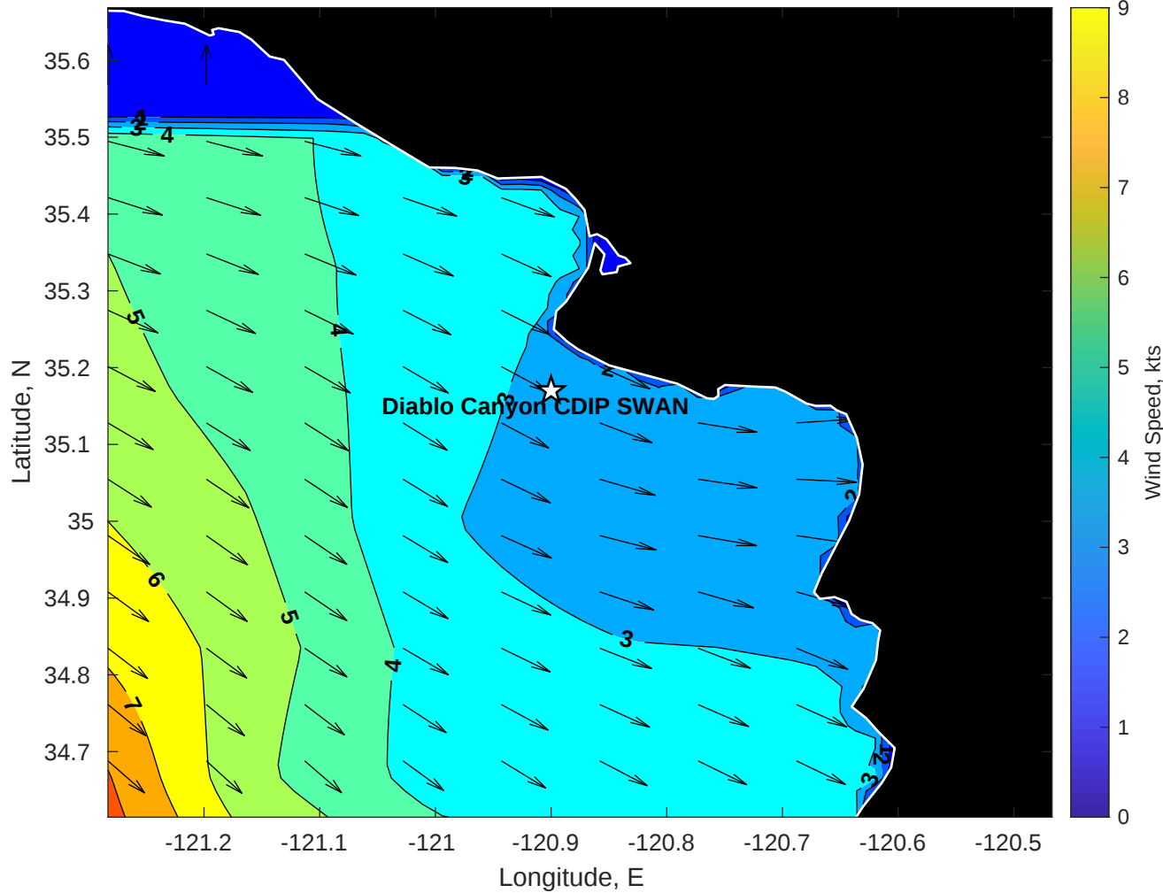
Winds (kts) for Diablo Canyon CDIP SWAN at 22-Oct-2025 08:00:00
