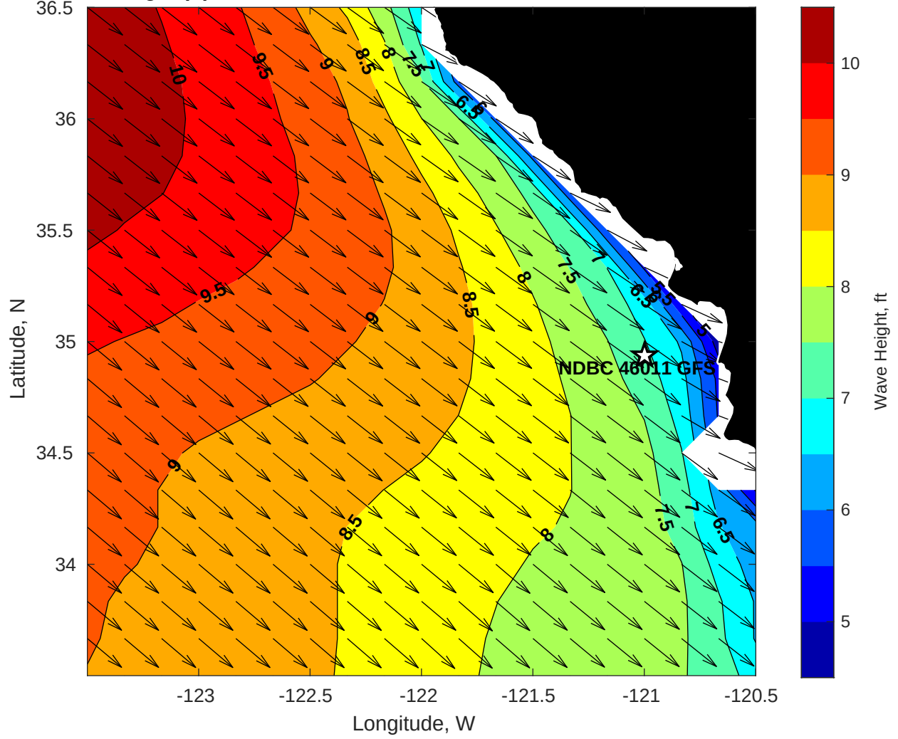
Wave Height (ft) for NDBC 46011 GFS at 22-Oct-2025 09:00:00
