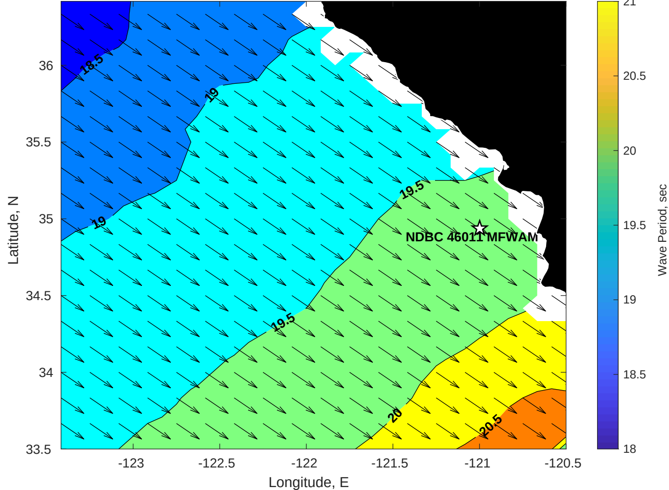
Wave Period (sec) for NDBC 46011 MFWAM at 22-Oct-2025 09:00:00
