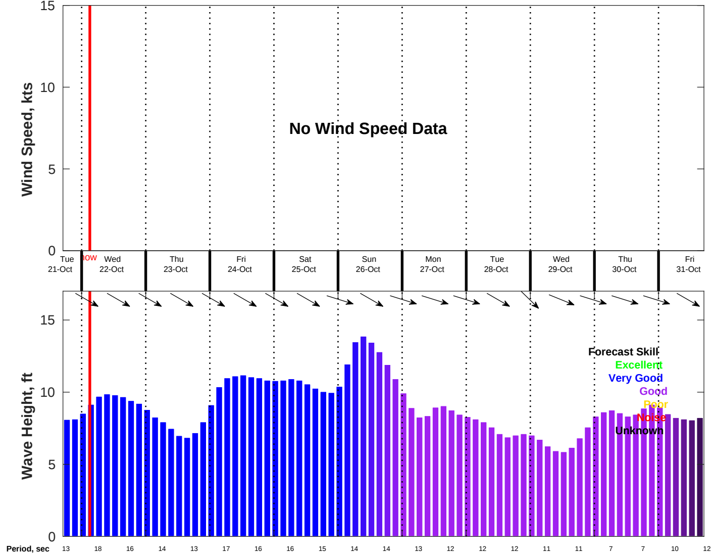
Wind & Wave Forecast for NDBC 46011 MFWAM from 21-Oct-2025 17:00:00 to 31-Oct-2025 17:00:00
