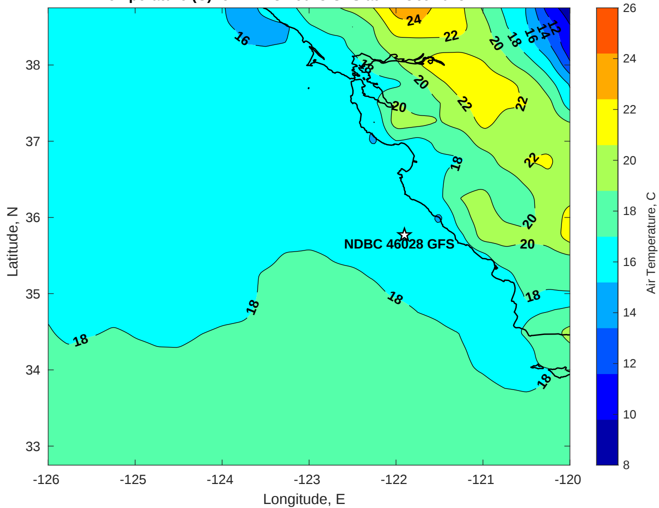
Air Temperature (C) for NDBC 46028 GFS at 22-Oct-2025
