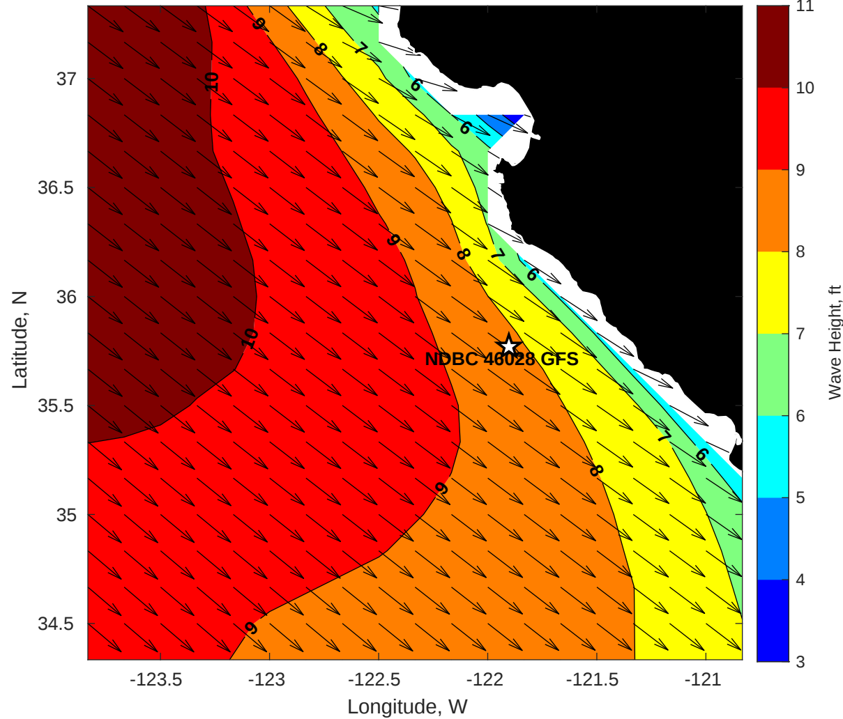
Wave Height (ft) for NDBC 46028 GFS at 22-Oct-2025 09:00:00
