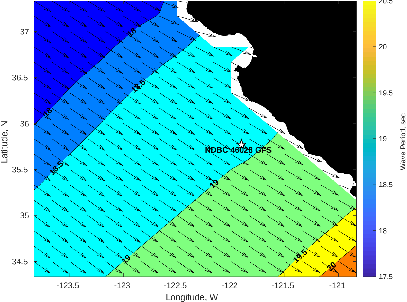
Wave Period (sec) for NDBC 46028 GFS at 22-Oct-2025 09:00:00
