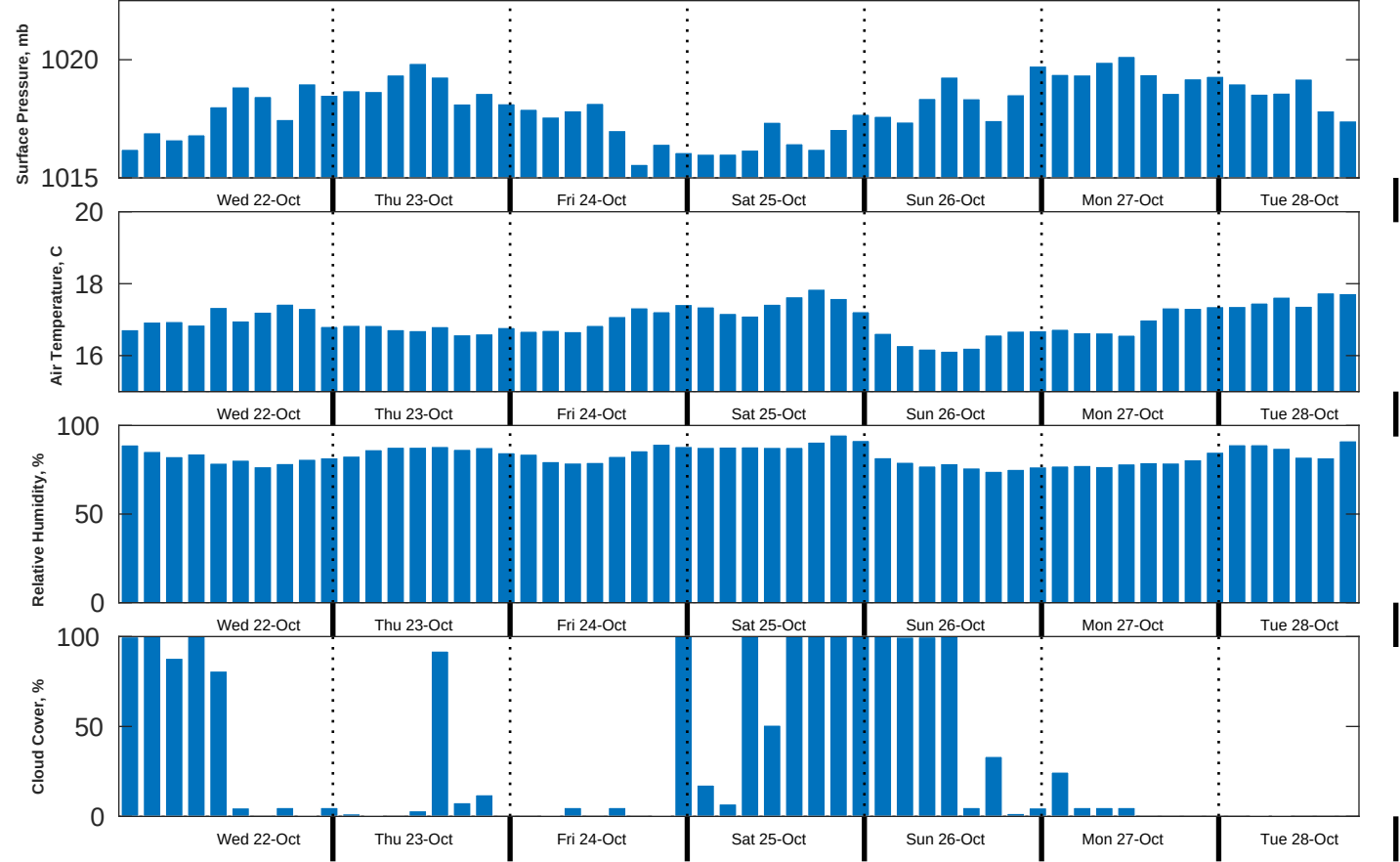
Met Forecast for NDBC 46028 GFS from 22-Oct-2025 00:00:00 to 29-Oct-2025 00:00:00
