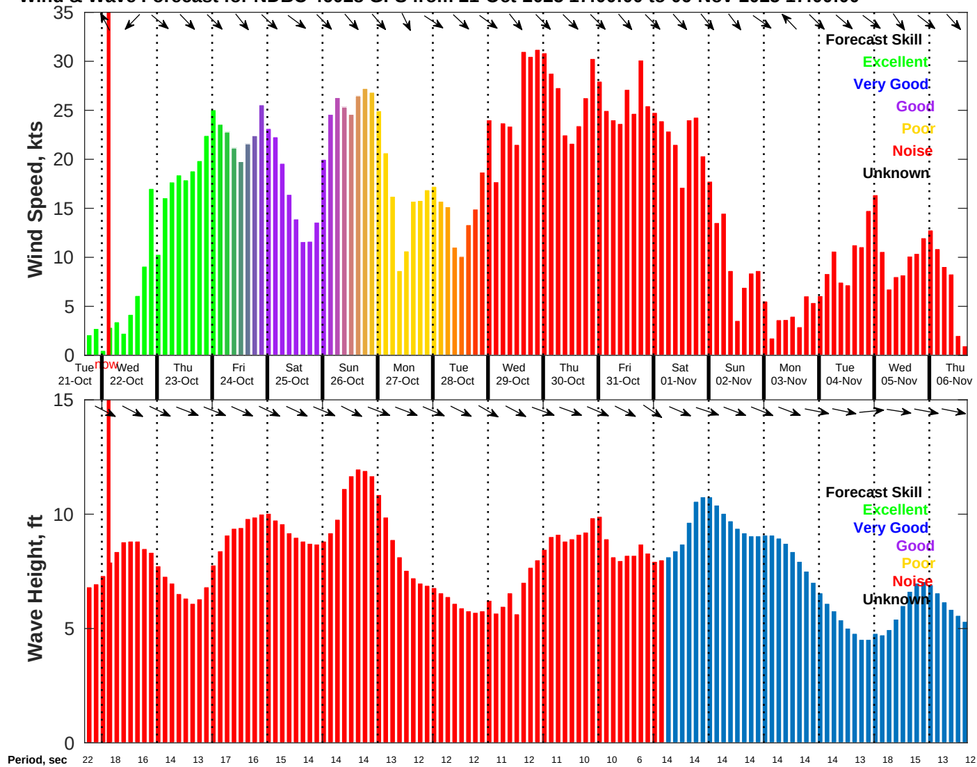
Wind & Wave Forecast for NDBC 46028 GFS from 21-Oct-2025 17:00:00 to 06-Nov-2025 17:00:00
