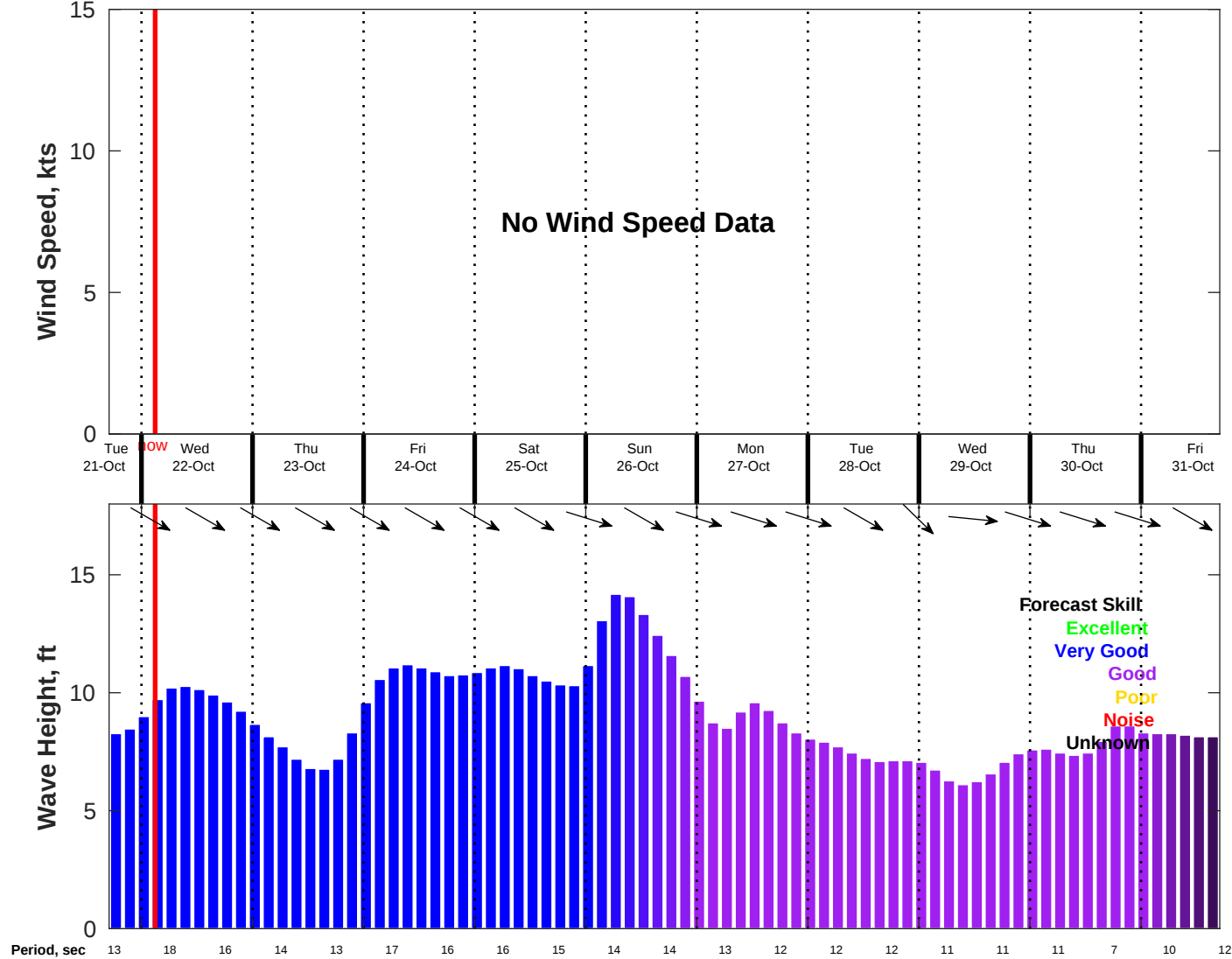
Wind & Wave Forecast for NDBC 46028 MFWAM from 21-Oct-2025 17:00:00 to 31-Oct-2025 17:00:00
