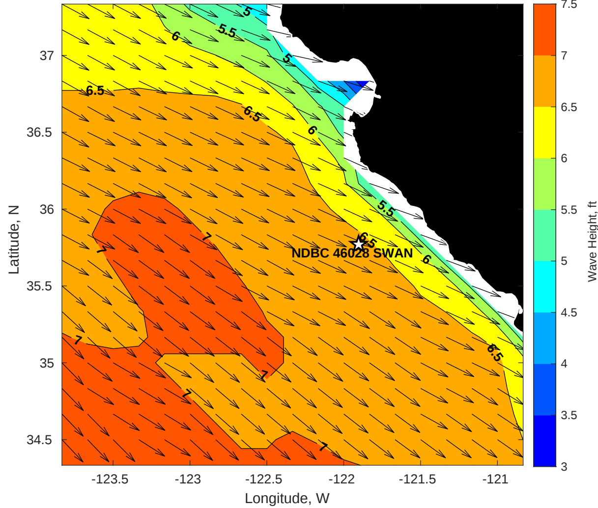
Wave Height (ft) for NDBC 46028 SWAN at 15-Nov-2025 21:00:00
