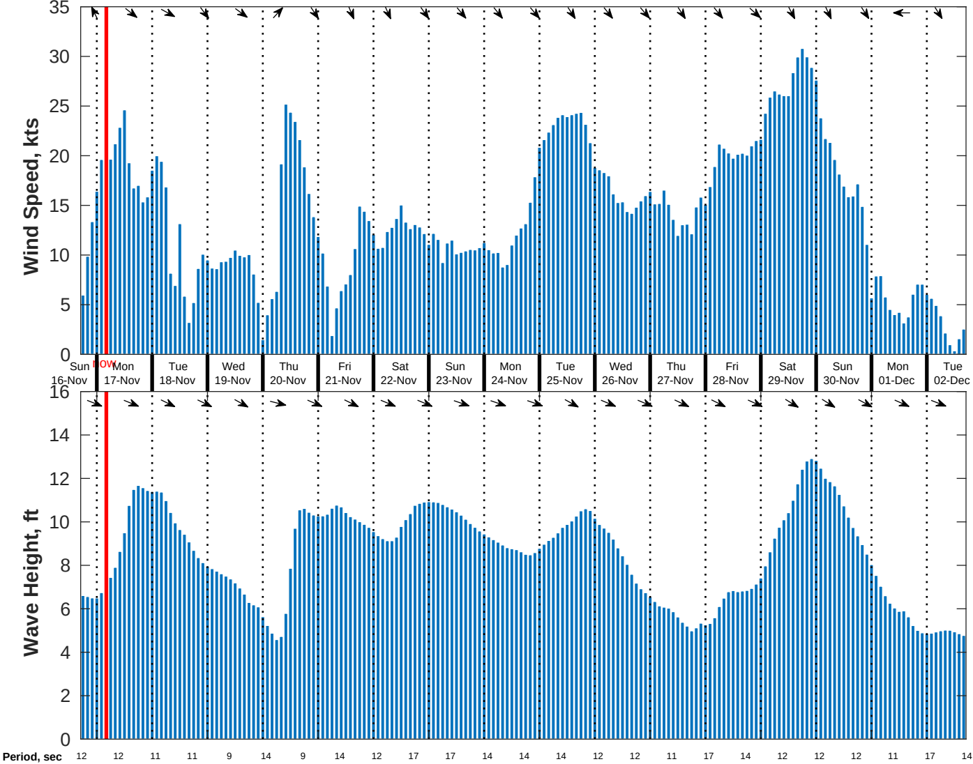
Wind & Wave Forecast for NDBC 46028 SWAN from 16-Nov-2025 17:00:00 to 02-Dec-2025 17:00:00
