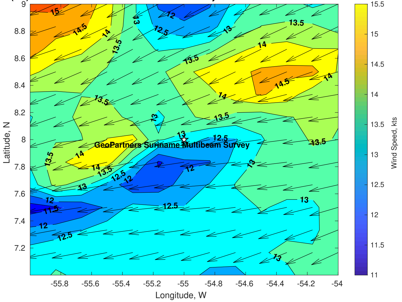
Winds (kts) for GeoPartners Suriname Multibeam Survey at 25-Dec-2024 09:00:00
