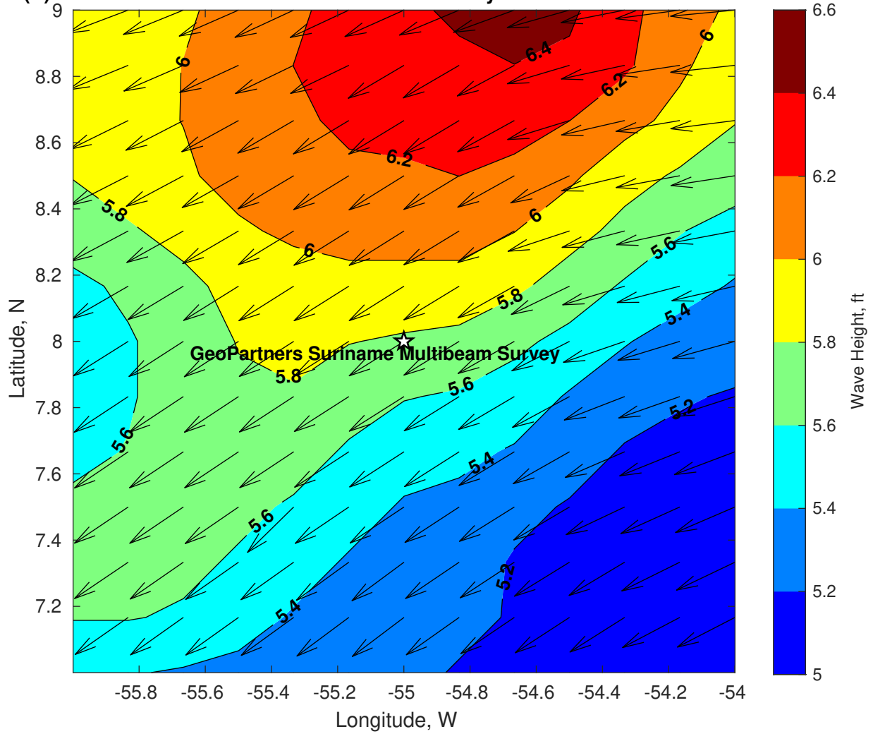
Wave Height (ft) for GeoPartners Suriname Multibeam Survey at 25-Dec-2024 09:00:00
