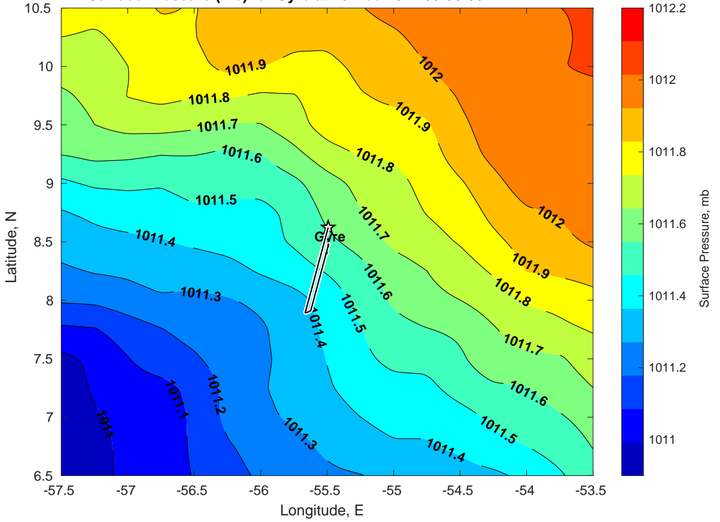
Surface Pressure (mb) for Gyre at 26-Dec-2024 00:00:00
