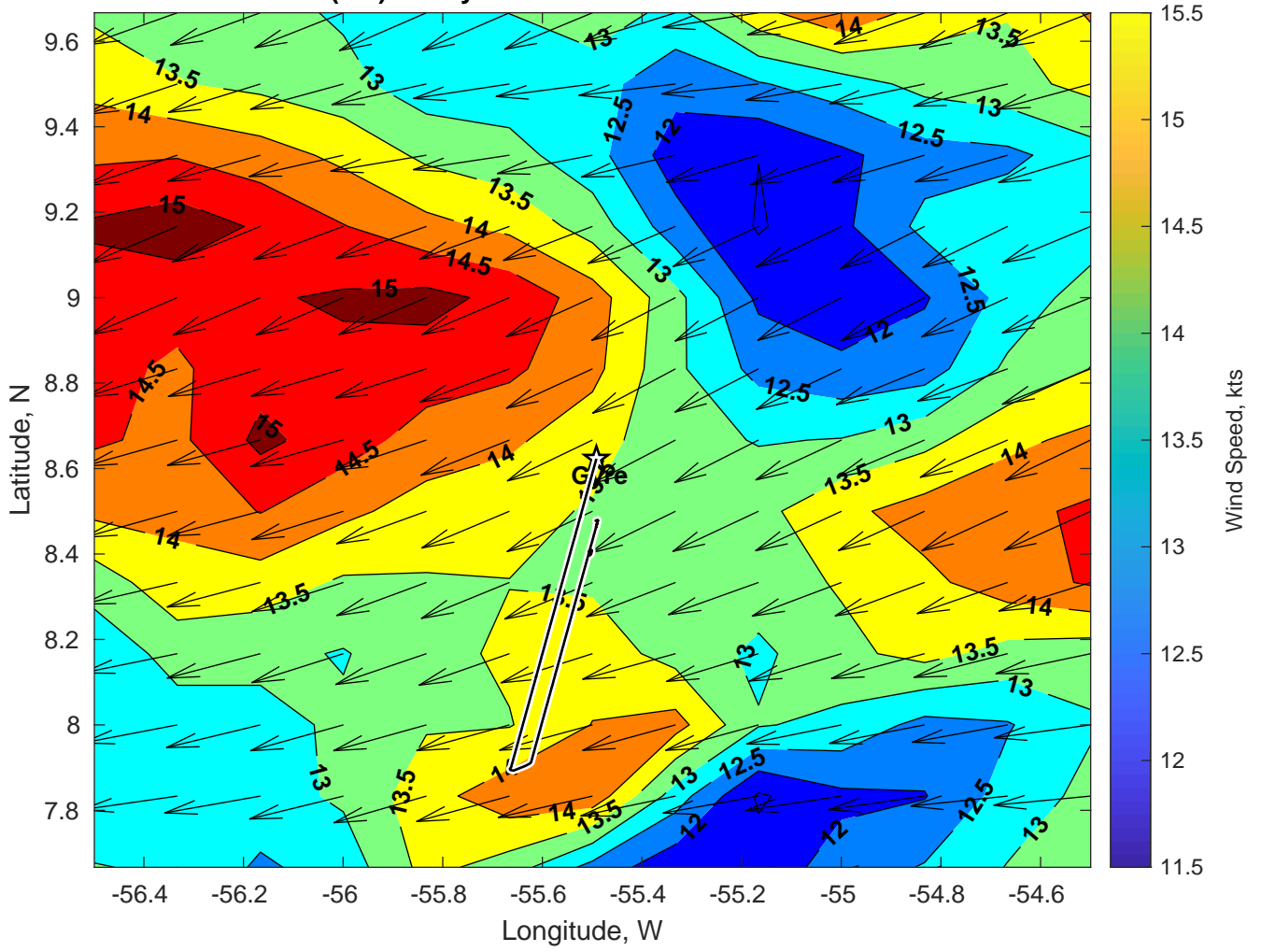
Winds (kts) for Gyre at 25-Dec-2024 09:00:00
