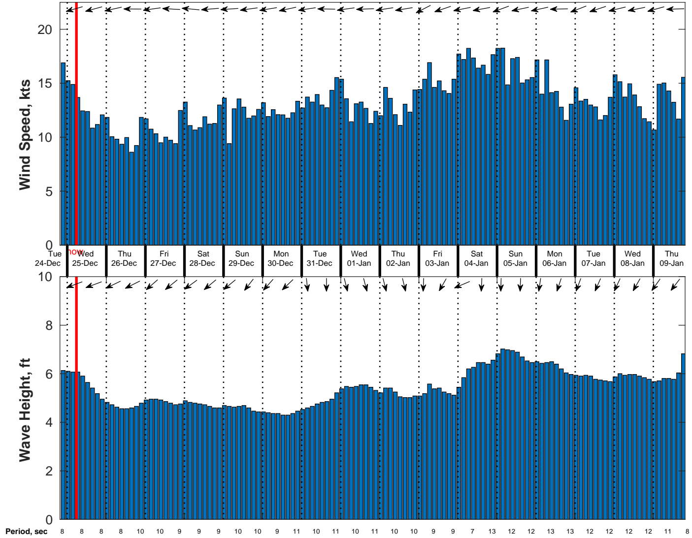
Wind & Wave Forecast for Gyre from 24-Dec-2024 20:00:00 to 09-Jan-2025 20:00:00
