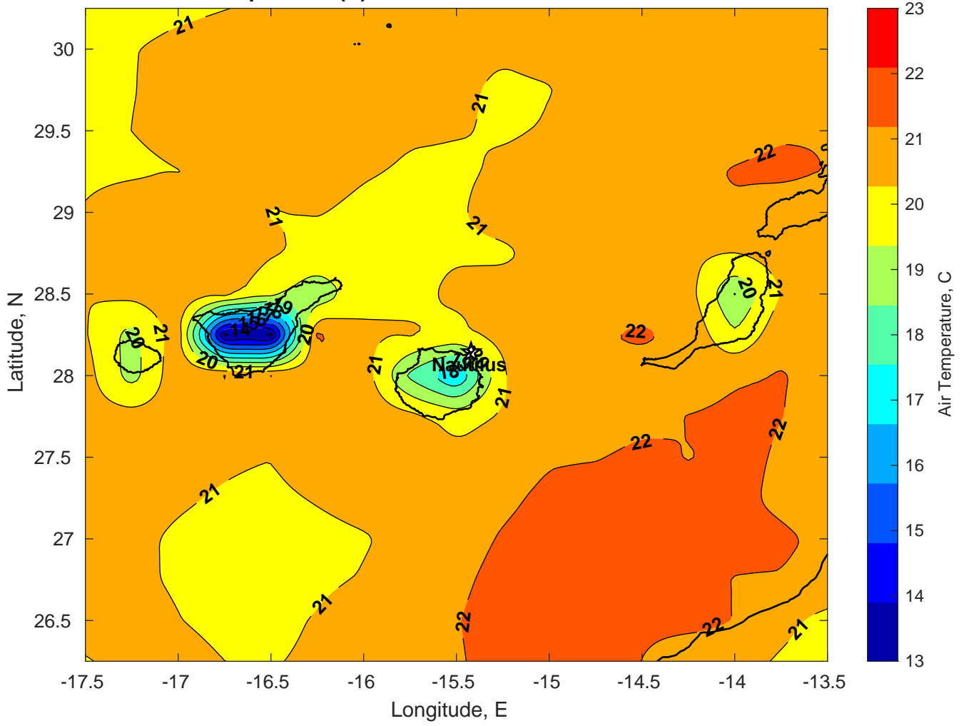
Air Temperature (C) for Nautilus at 25-Dec-2024
