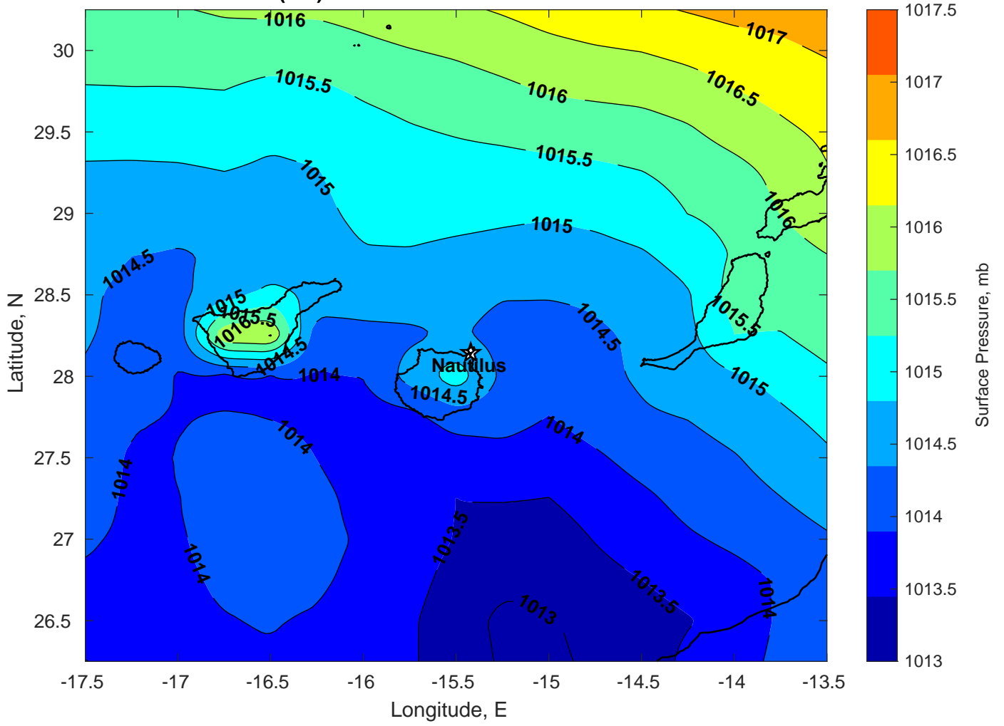
Surface Pressure (mb) for Nautilus at 25-Dec-2024 00:00:00
