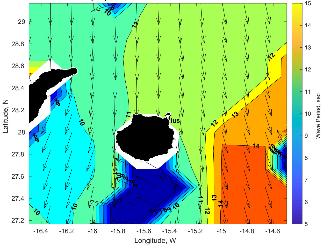
Wave Period (sec) for Nautilus at 25-Dec-2024 09:00:00
