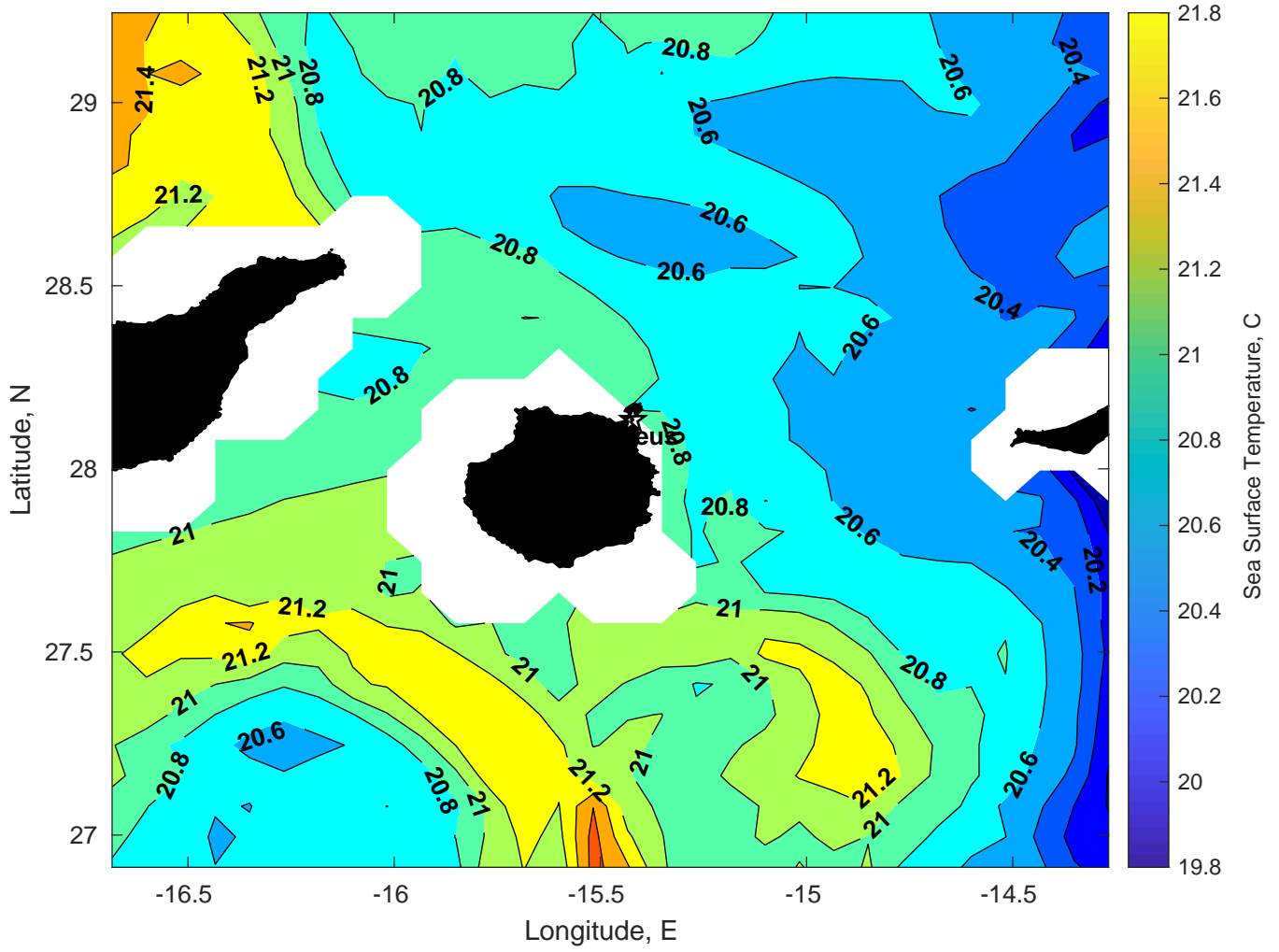
SST for Proteus at 24-Dec-2024 00:00:00
