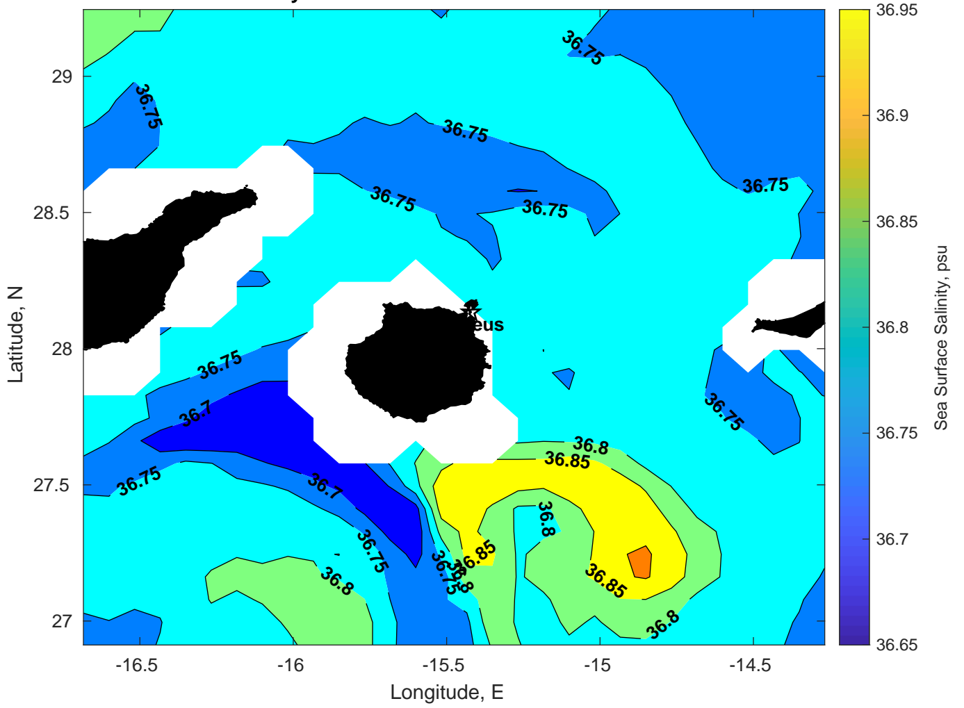
Surface Salinity for Proteus at 24-Dec-2024 00:00:00
