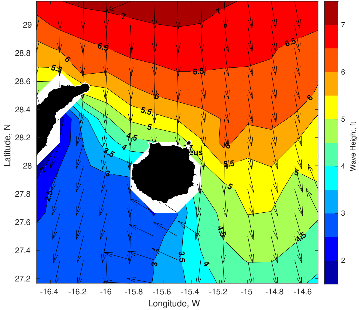
Wave Height (ft) for Proteus at 25-Dec-2024 09:00:00
