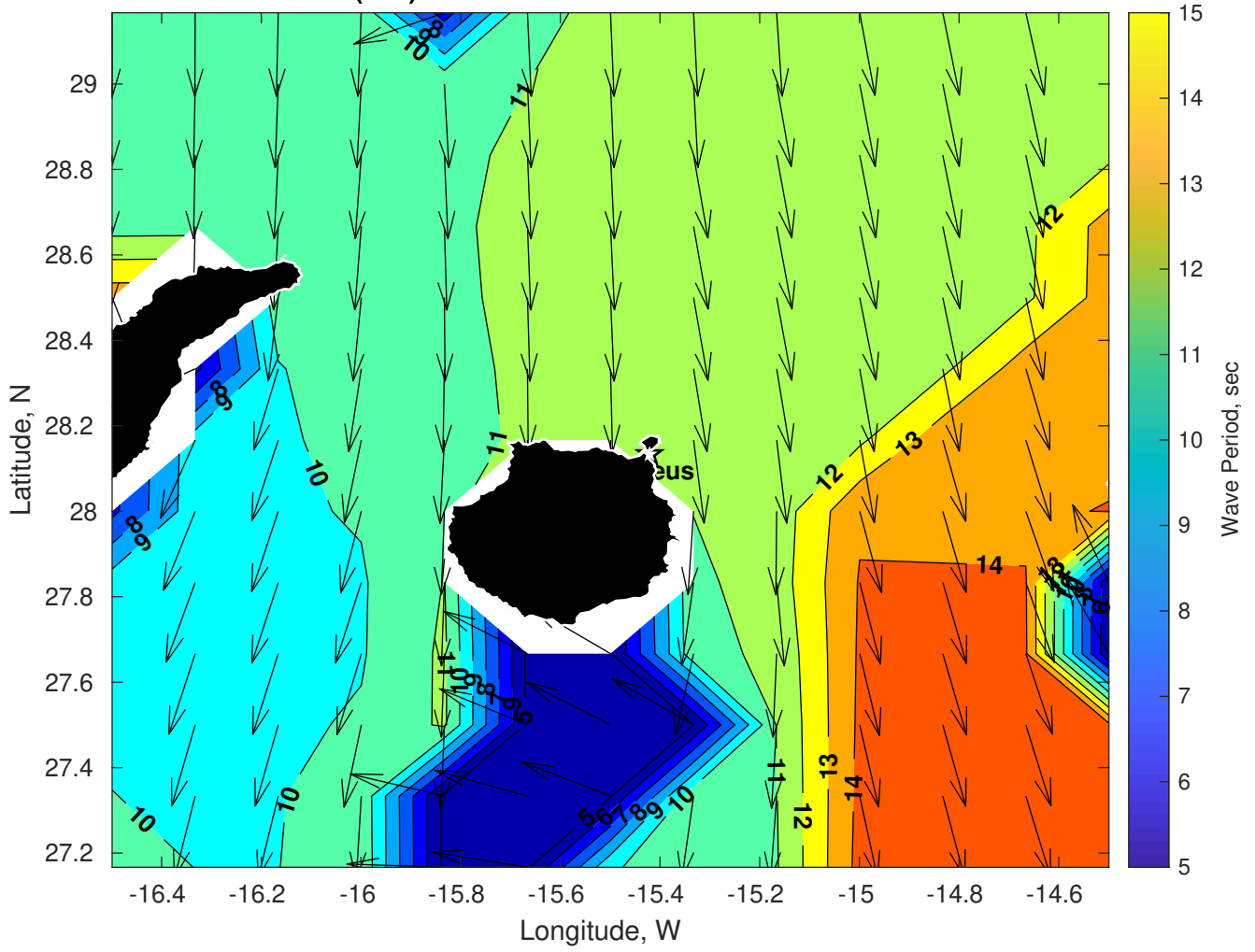
Wave Period (sec) for Proteus at 25-Dec-2024 09:00:00
