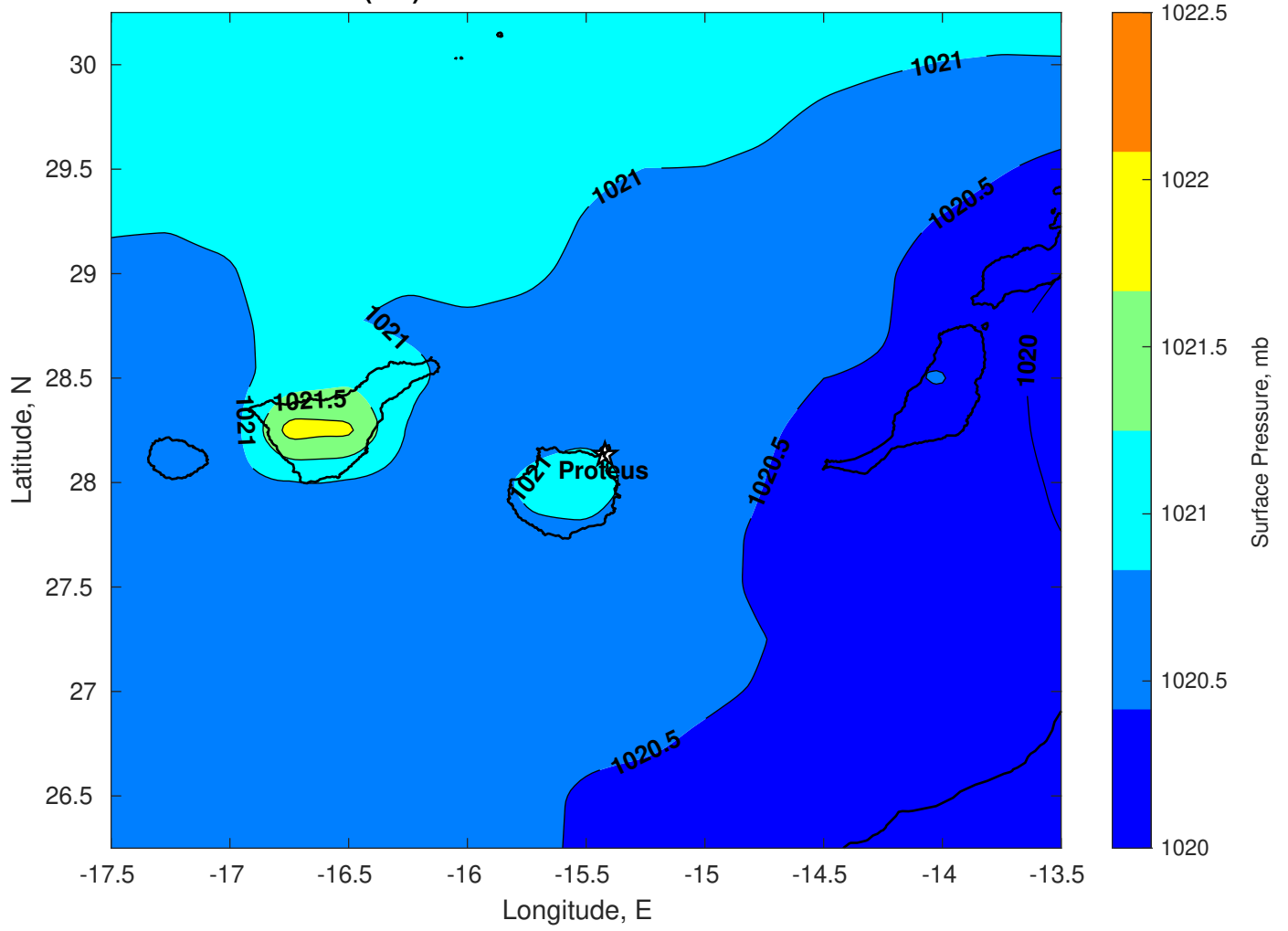
Surface Pressure (mb) for Proteus at 27-Dec-2024 00:00:00
