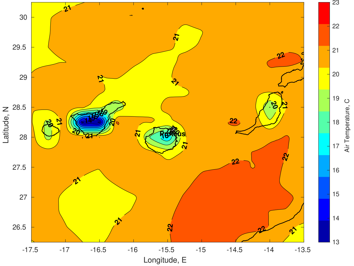
Air Temperature (C) for Proteus at 25-Dec-2024
