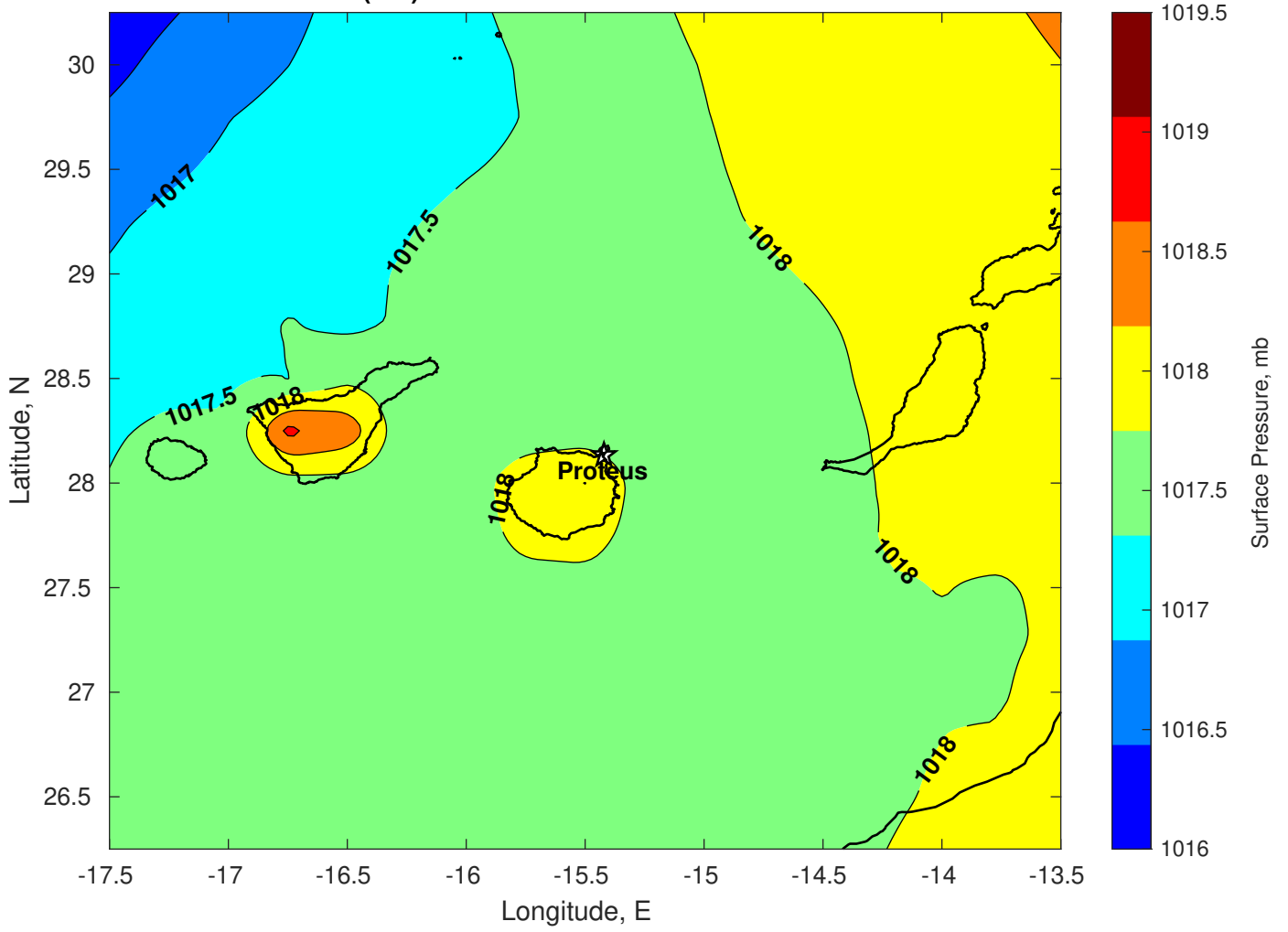
Surface Pressure (mb) for Proteus at 26-Dec-2024 00:00:00
