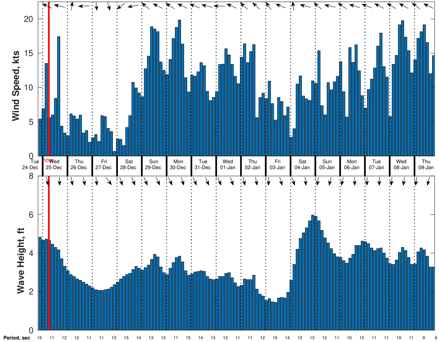
Wind & Wave Forecast for Proteus from 24-Dec-2024 20:00:00 to 09-Jan-2025 20:00:00
