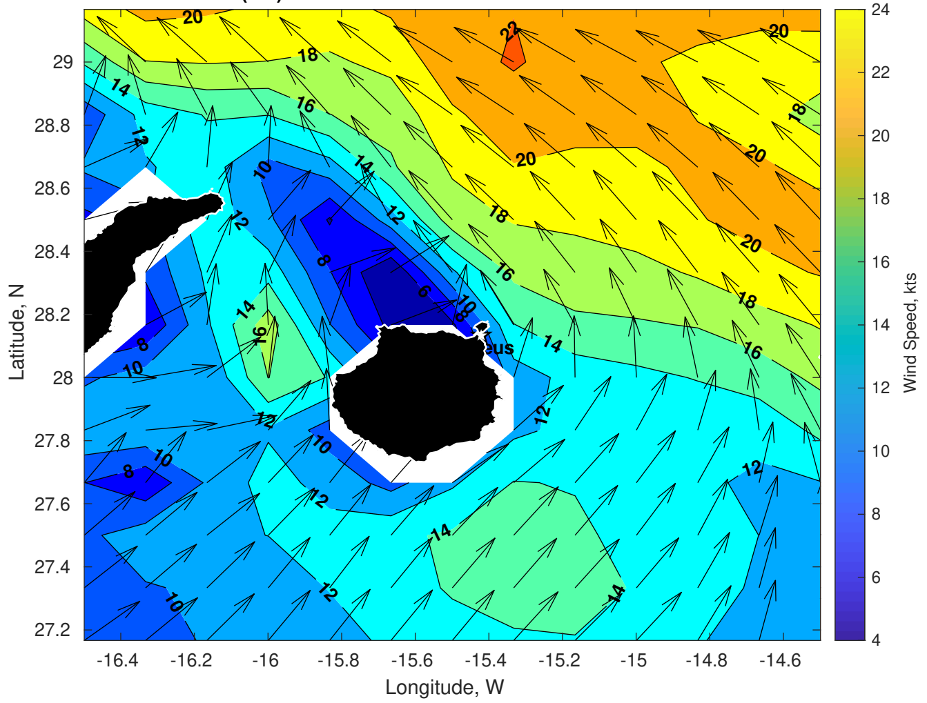
Winds (kts) for Proteus at 25-Dec-2024 09:00:00
