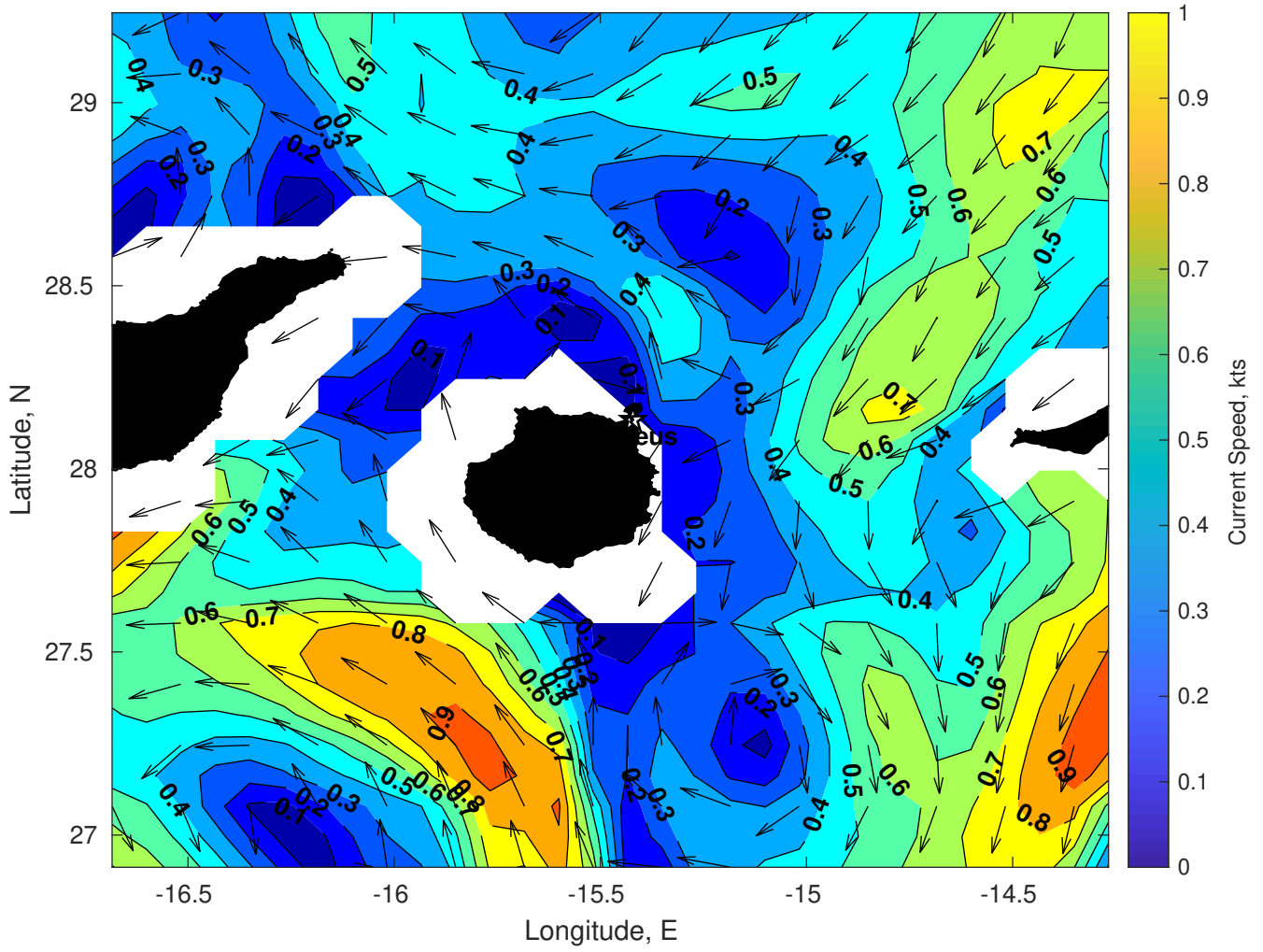
Surface Currents for Proteus at 24-Dec-2024 00:00:00
