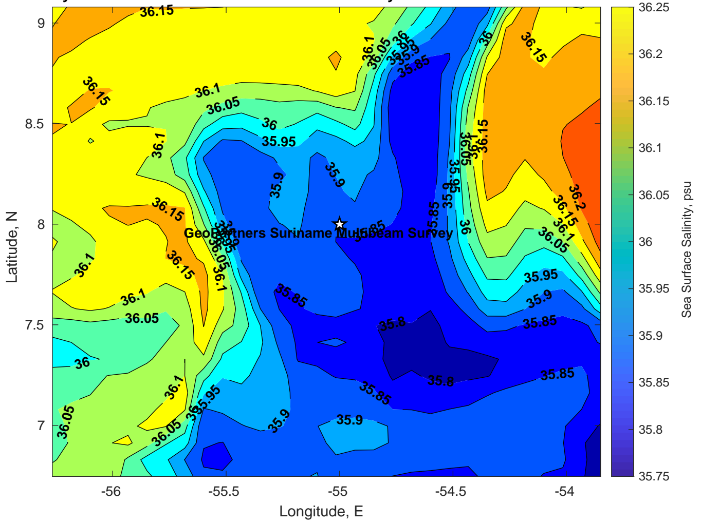
Surface Salinity for GeoPartners Suriname Multibeam Survey at 25-Dec-2024 00:00:00
