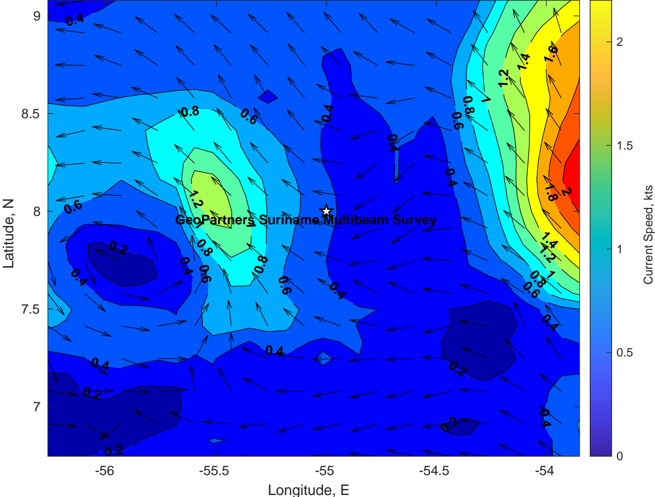
Surface Currents for GeoPartners Suriname Multibeam Survey at 25-Dec-2024 00:00:00
