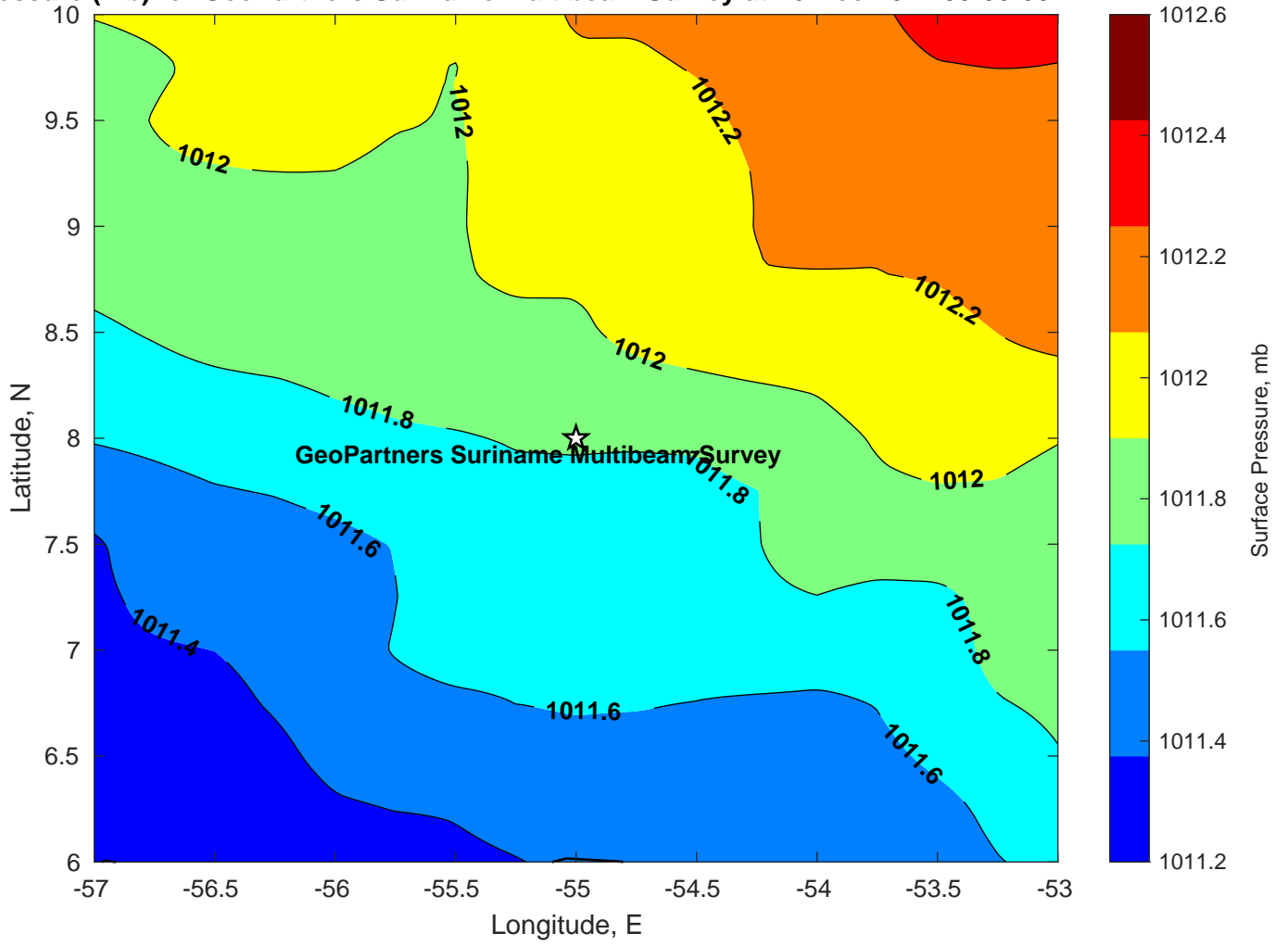
Surface Pressure (mb) for GeoPartners Suriname Multibeam Survey at 26-Dec-2024 00:00:00
