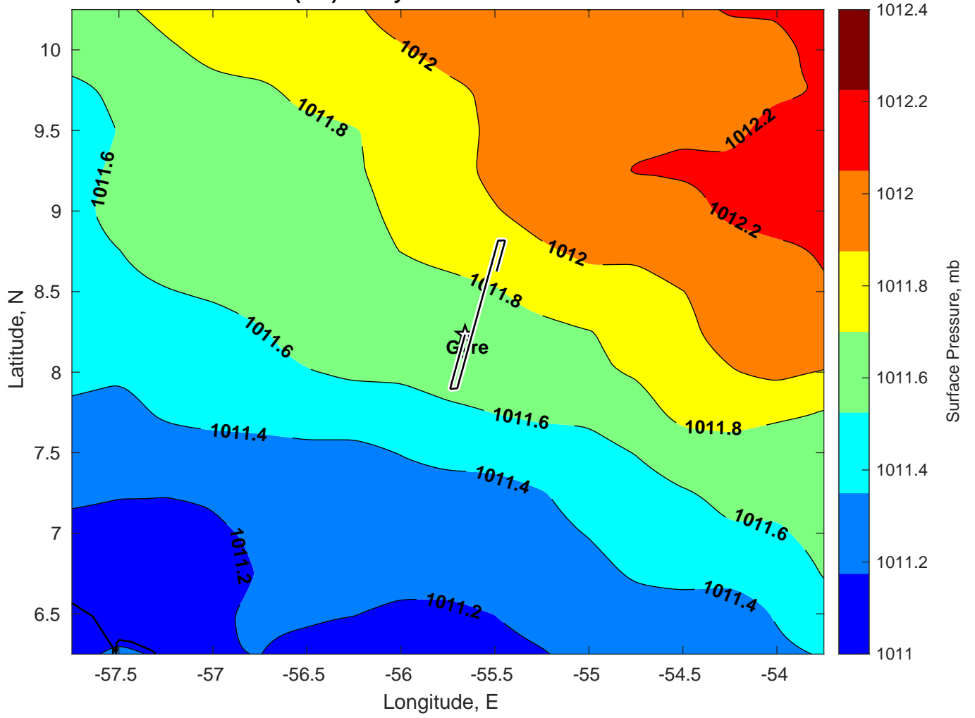
Surface Pressure (mb) for Gyre at 27-Dec-2024 00:00:00
