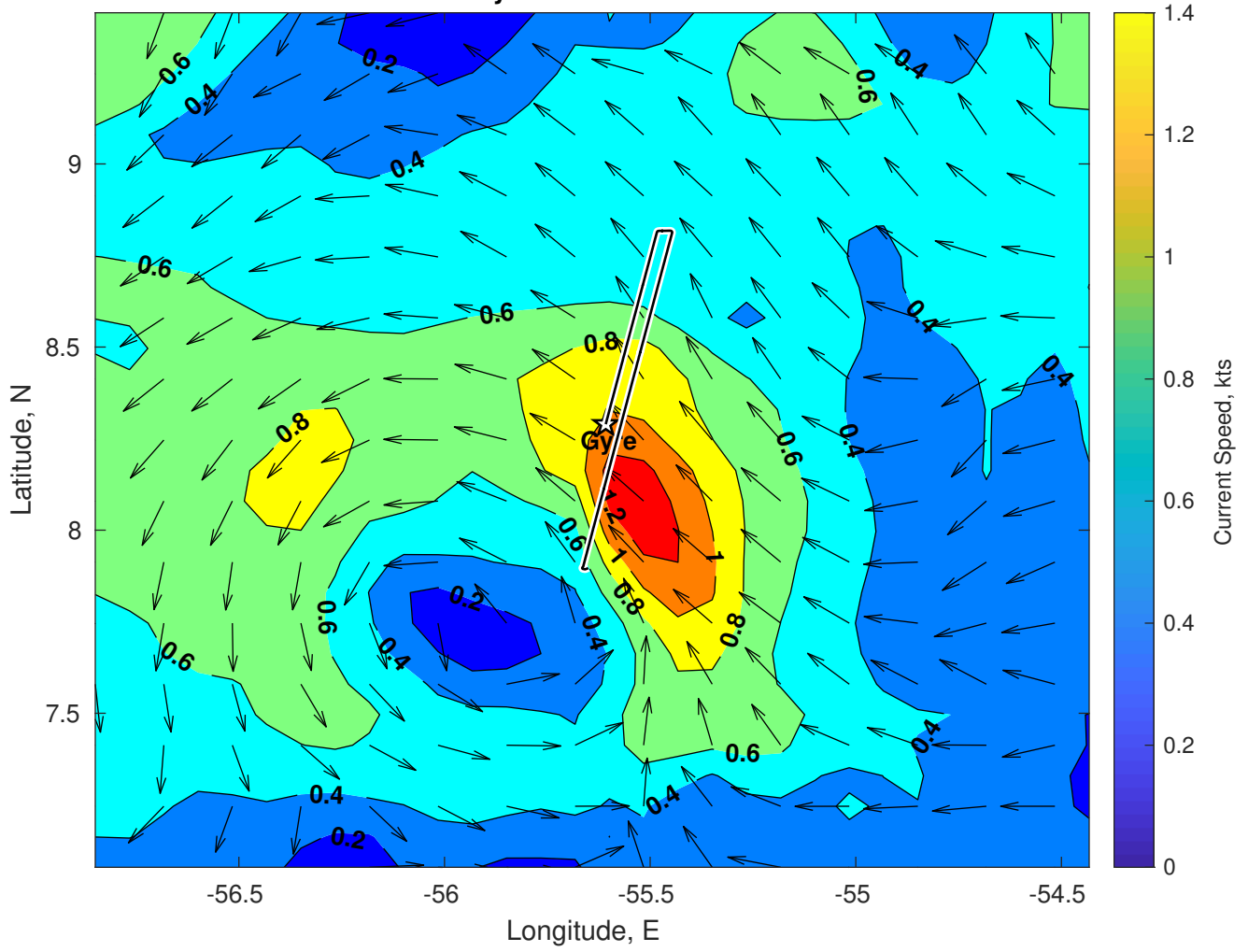
Surface Currents for Gyre at 25-Dec-2024 00:00:00
