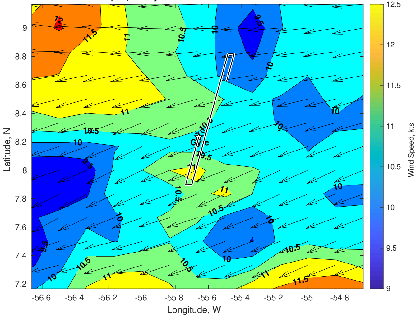
Winds (kts) for Gyre at 26-Dec-2024 09:00:00
