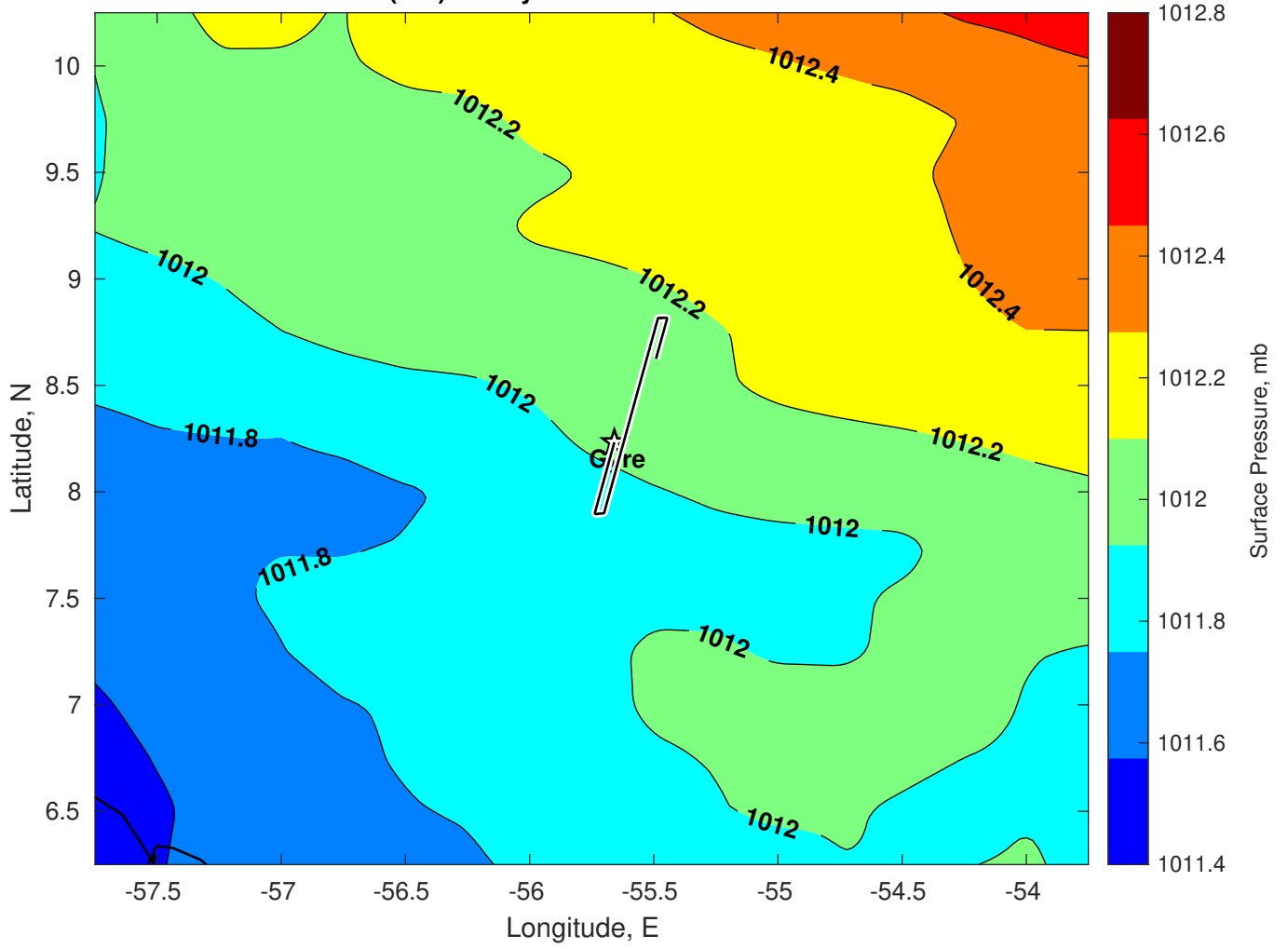
Surface Pressure (mb) for Gyre at 28-Dec-2024 00:00:00
