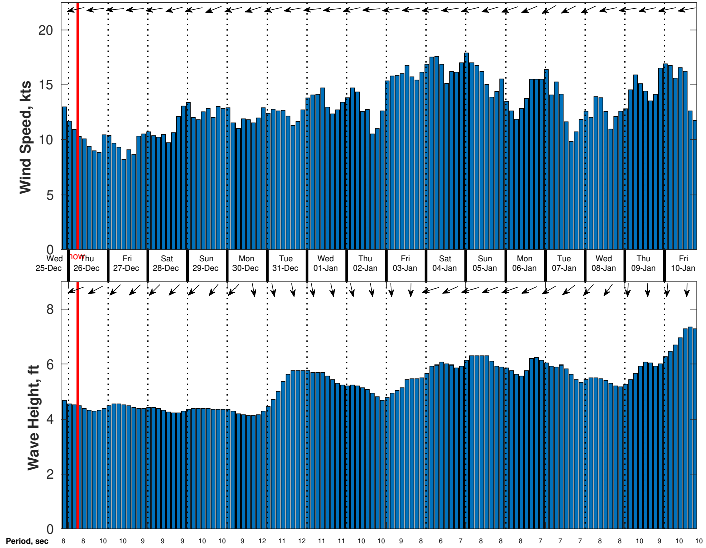
Wind & Wave Forecast for Gyre from 25-Dec-2024 20:00:00 to 10-Jan-2025 20:00:00
