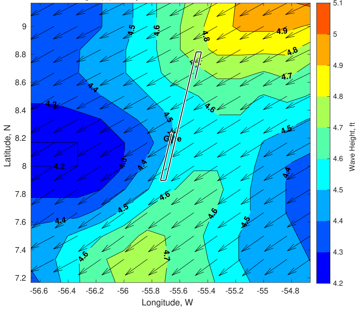
Wave Height (ft) for Gyre at 26-Dec-2024 09:00:00
