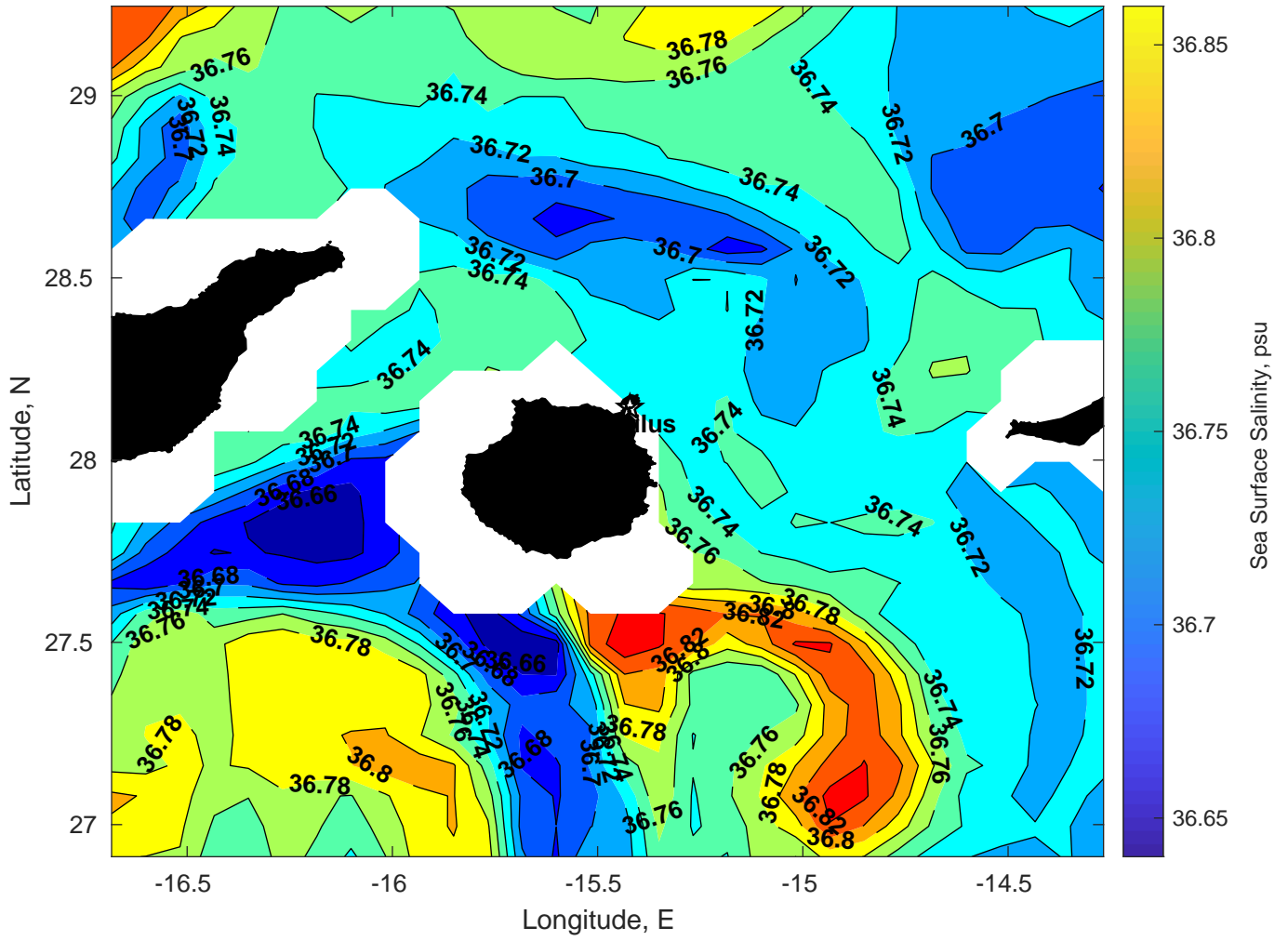
Surface Salinity for Nautilus at 25-Dec-2024 00:00:00
