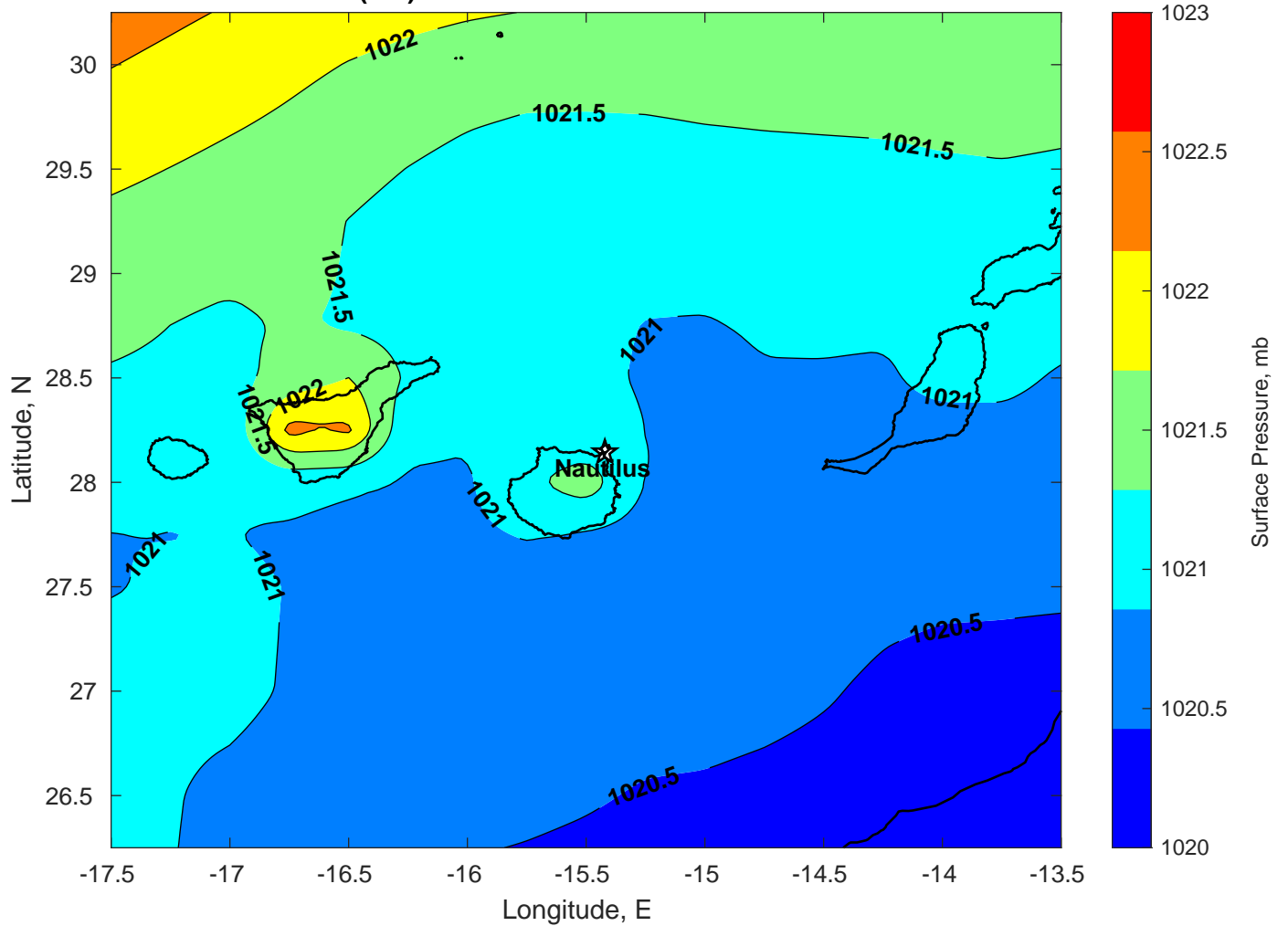
Surface Pressure (mb) for Nautilus at 28-Dec-2024 00:00:00
