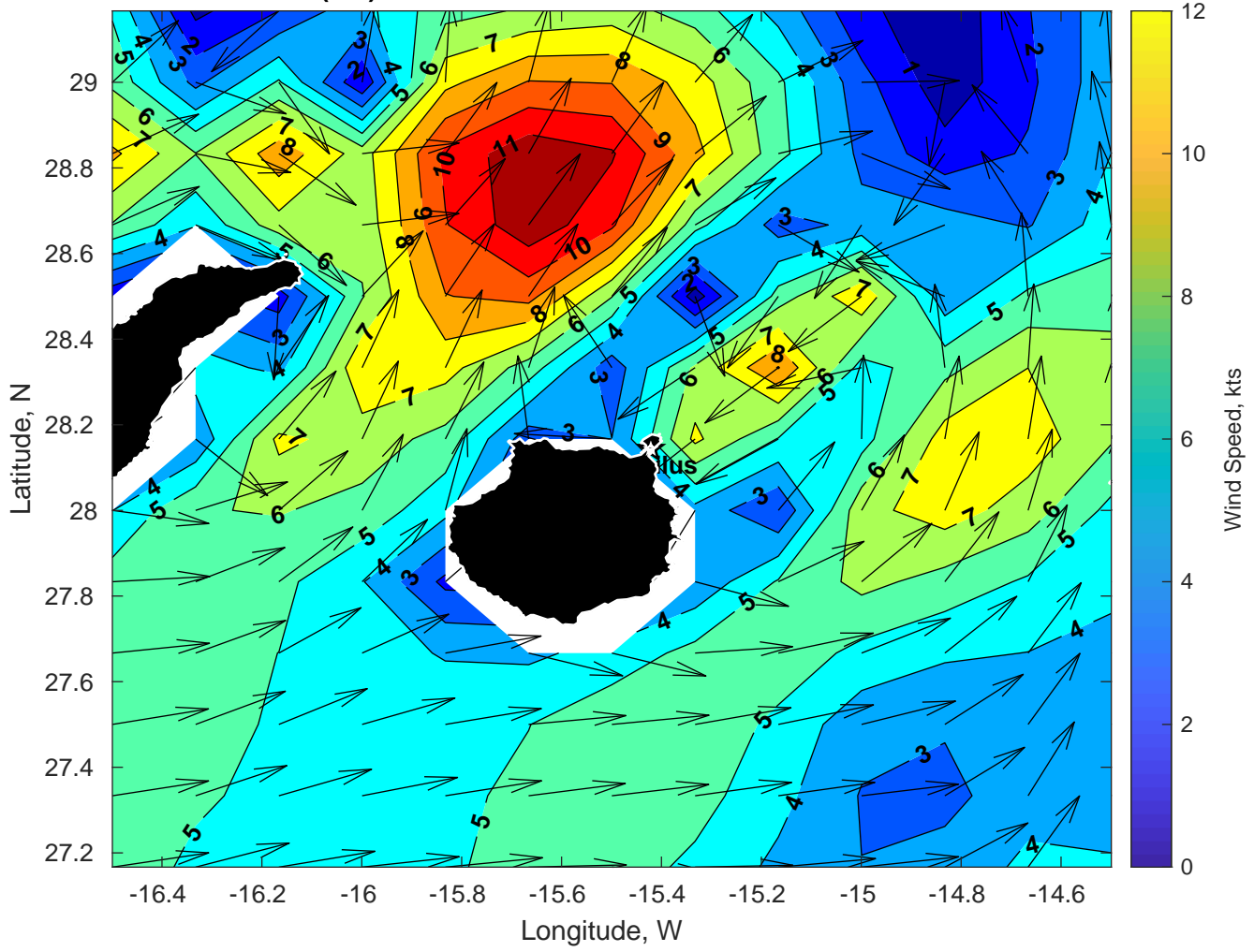
Winds (kts) for Nautilus at 26-Dec-2024 09:00:00
