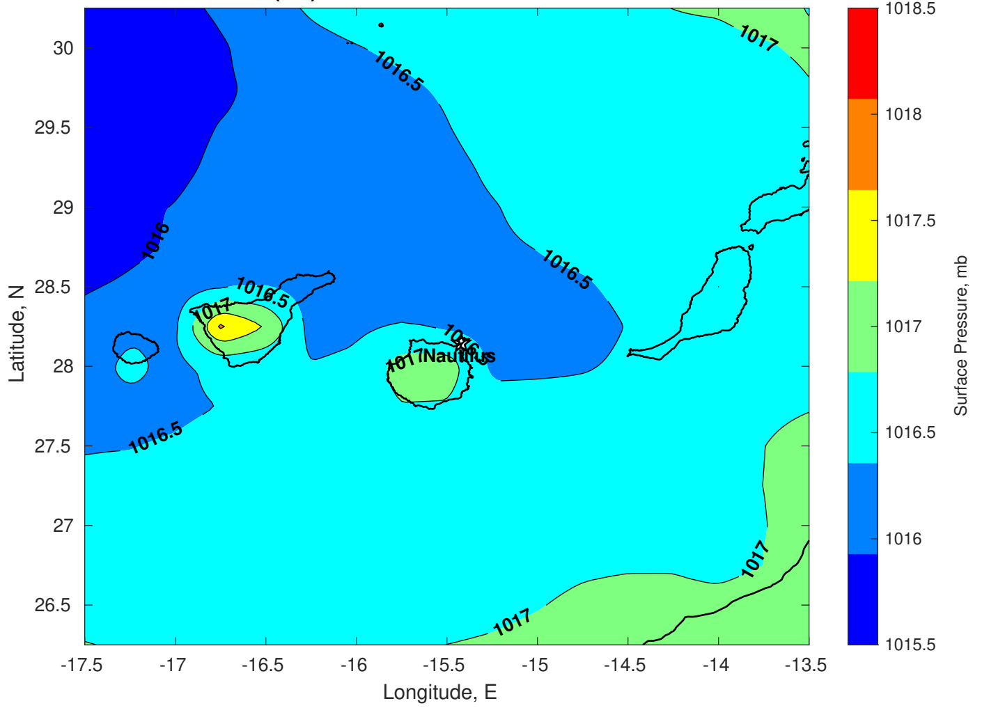
Surface Pressure (mb) for Nautilus at 26-Dec-2024 00:00:00
