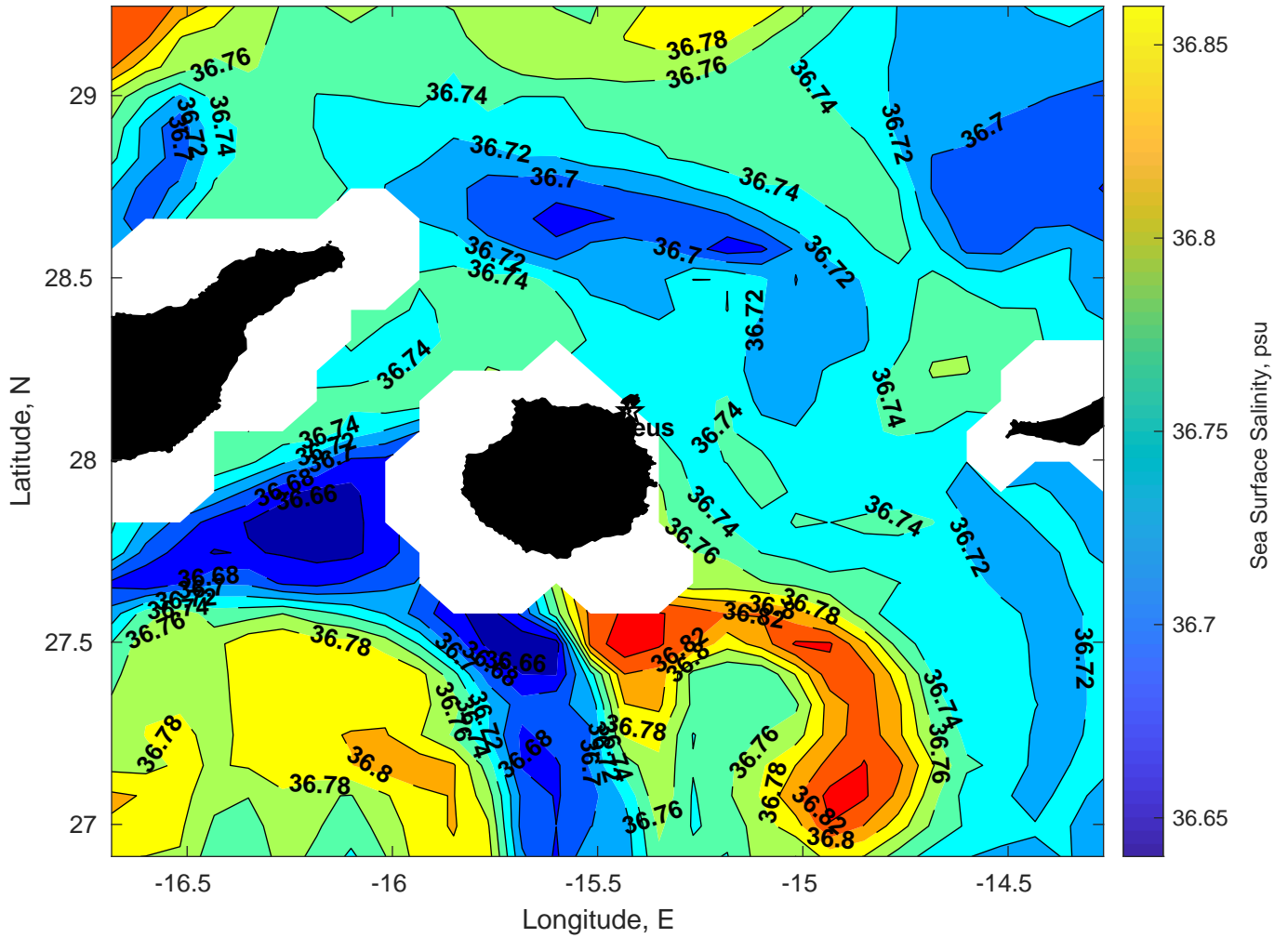
Surface Salinity for Proteus at 25-Dec-2024 00:00:00
