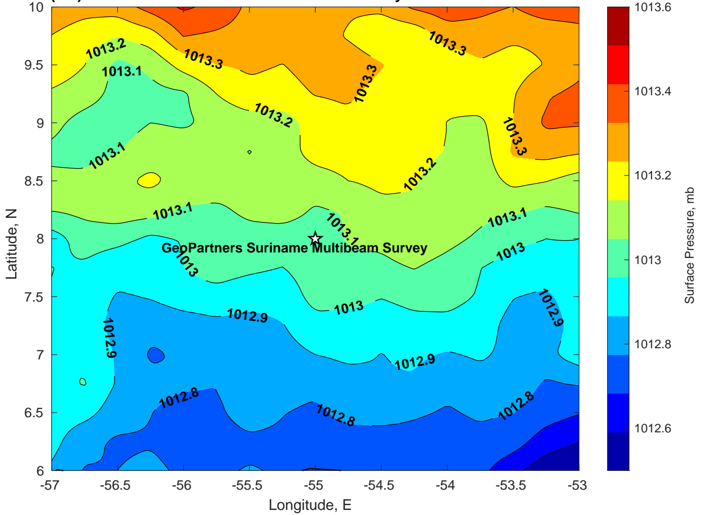
Surface Pressure (mb) for GeoPartners Suriname Multibeam Survey at 26-Dec-2024 12:00:00
