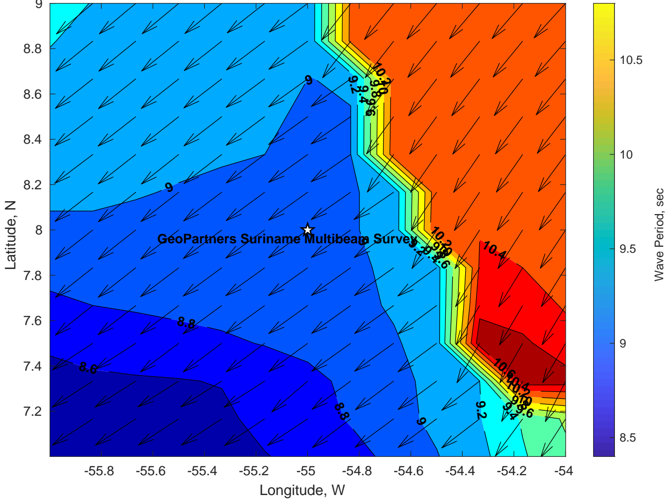
Wave Period (sec) for GeoPartners Suriname Multibeam Survey at 26-Dec-2024 21:00:00
