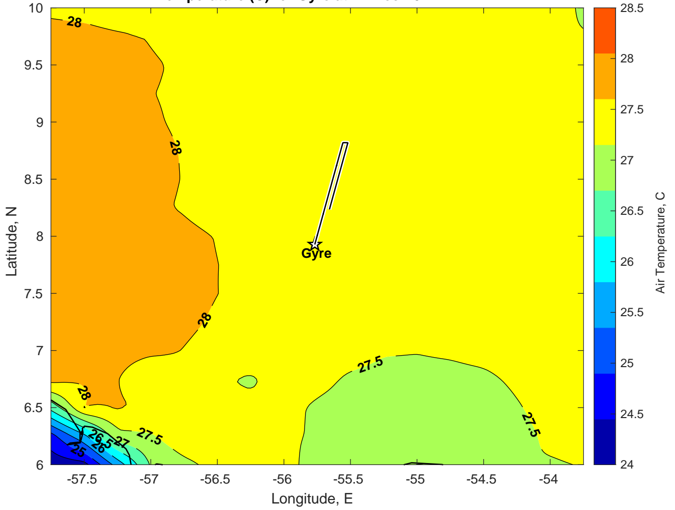
Air Temperature (C) for Gyre at 27-Dec-2024
