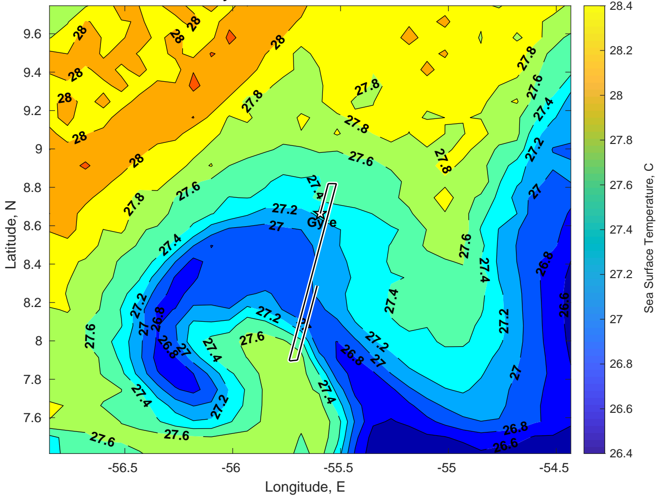
SST for Gyre at 26-Dec-2024 00:00:00
