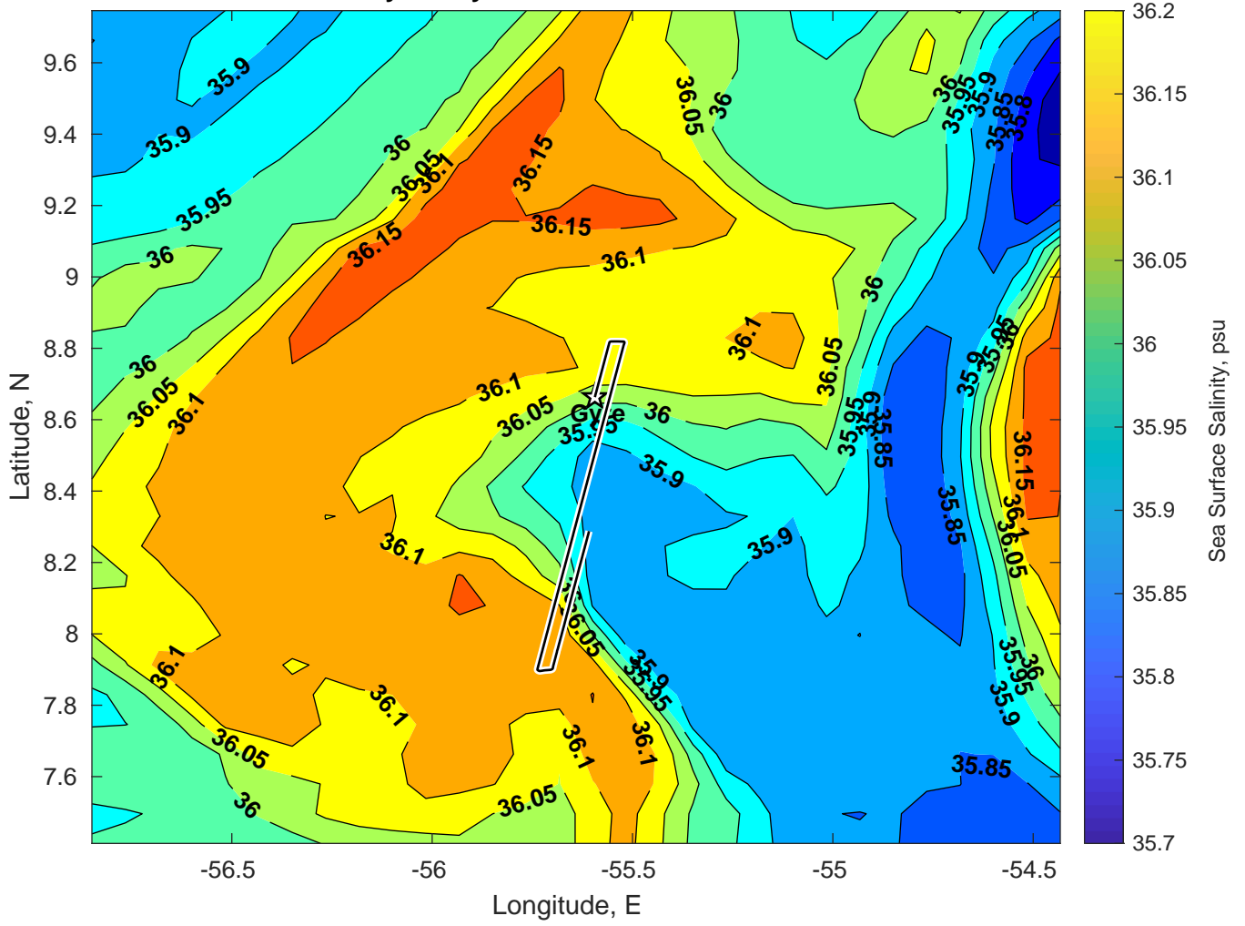
Surface Salinity for Gyre at 26-Dec-2024 00:00:00
