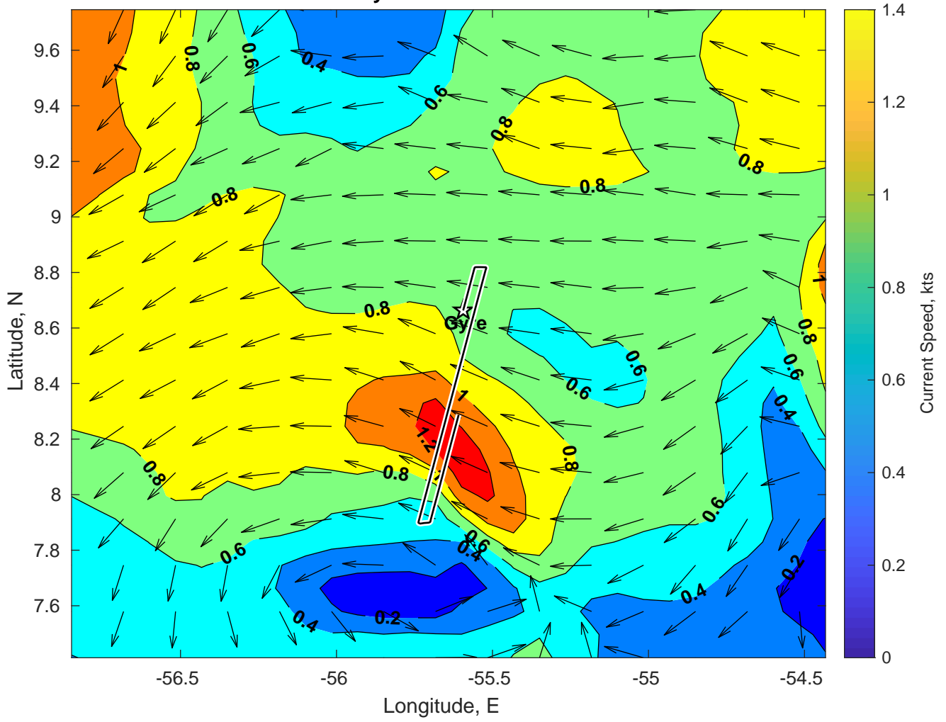
Surface Currents for Gyre at 26-Dec-2024 00:00:00
