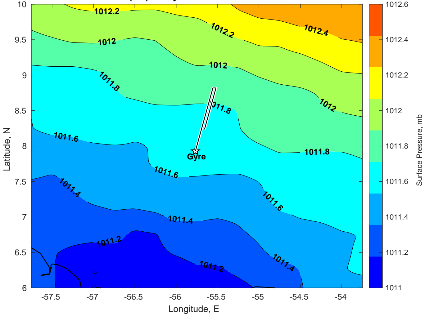
Surface Pressure (mb) for Gyre at 29-Dec-2024 00:00:00
