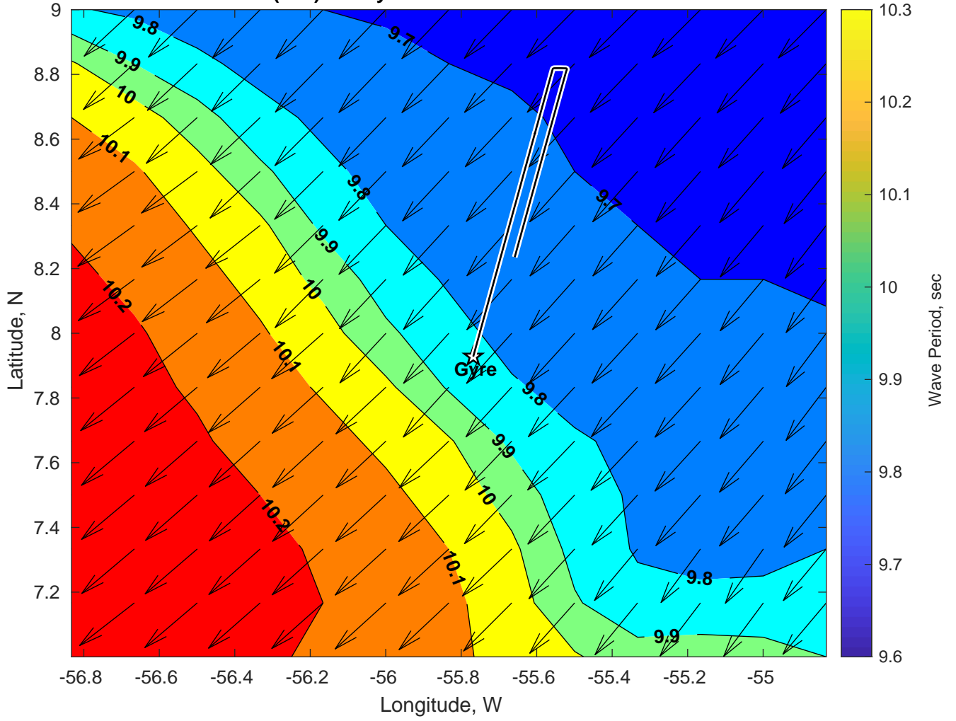
Wave Period (sec) for Gyre at 27-Dec-2024 09:00:00
