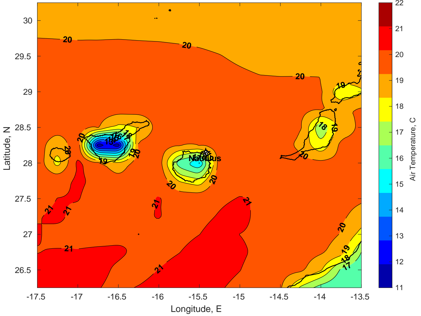
Air Temperature (C) for Nautilus at 27-Dec-2024
