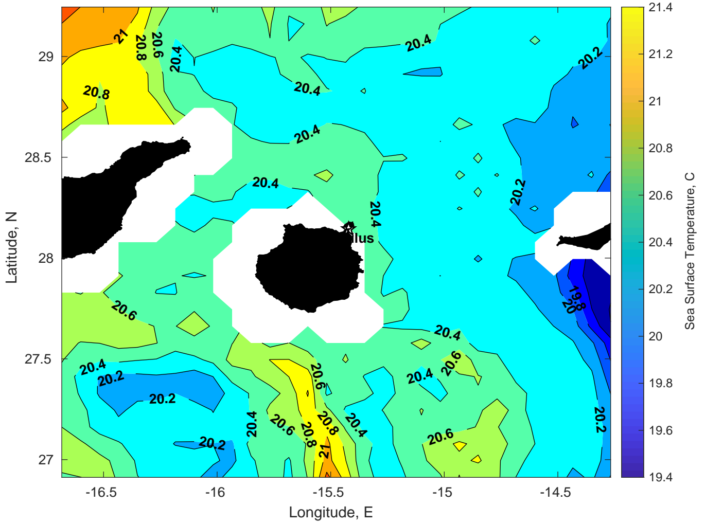
SST for Nautilus at 26-Dec-2024 00:00:00
