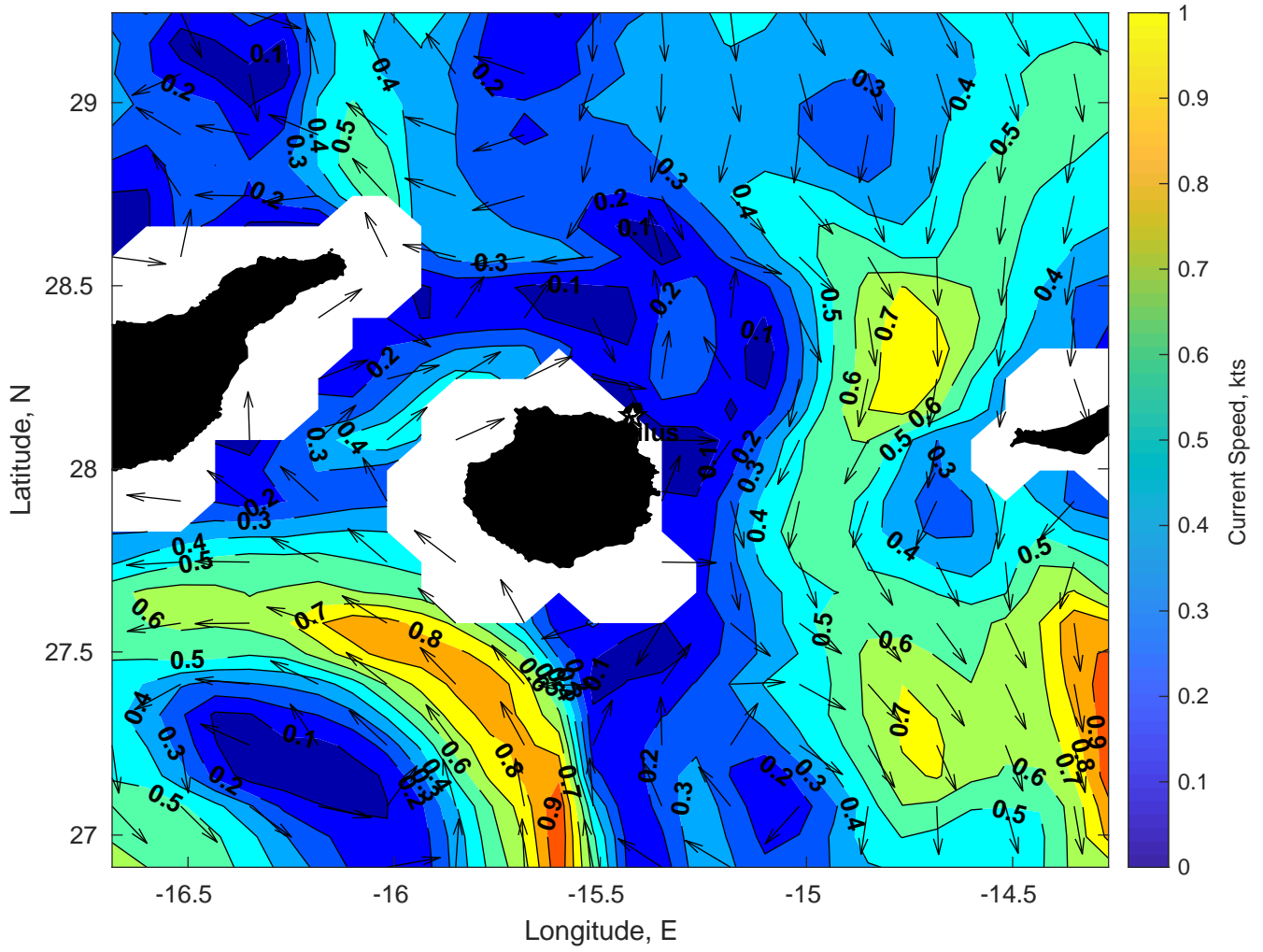
Surface Currents for Nautilus at 26-Dec-2024 00:00:00
