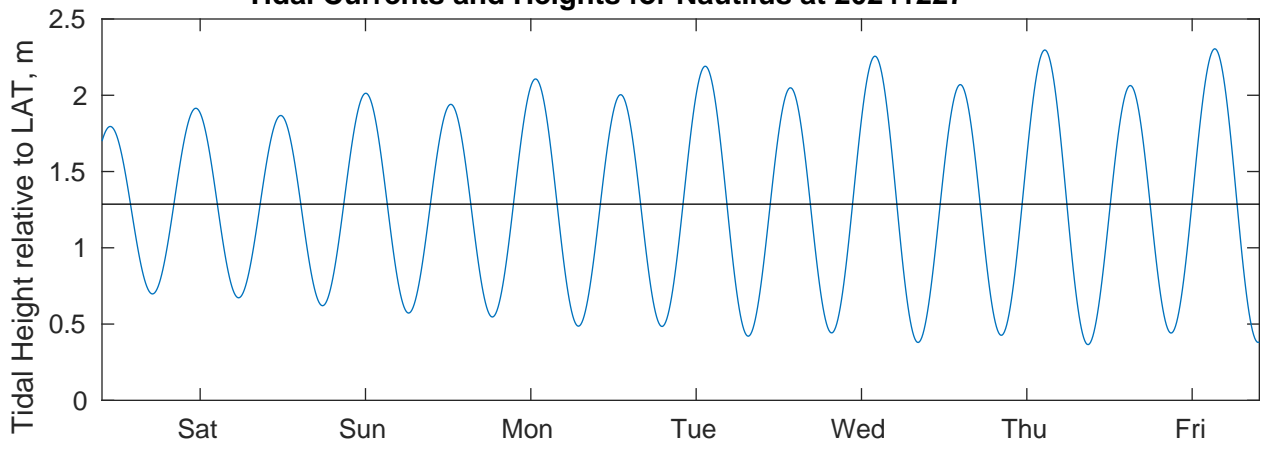
Tidal Currents and Heights for Nautilus at 20241227
