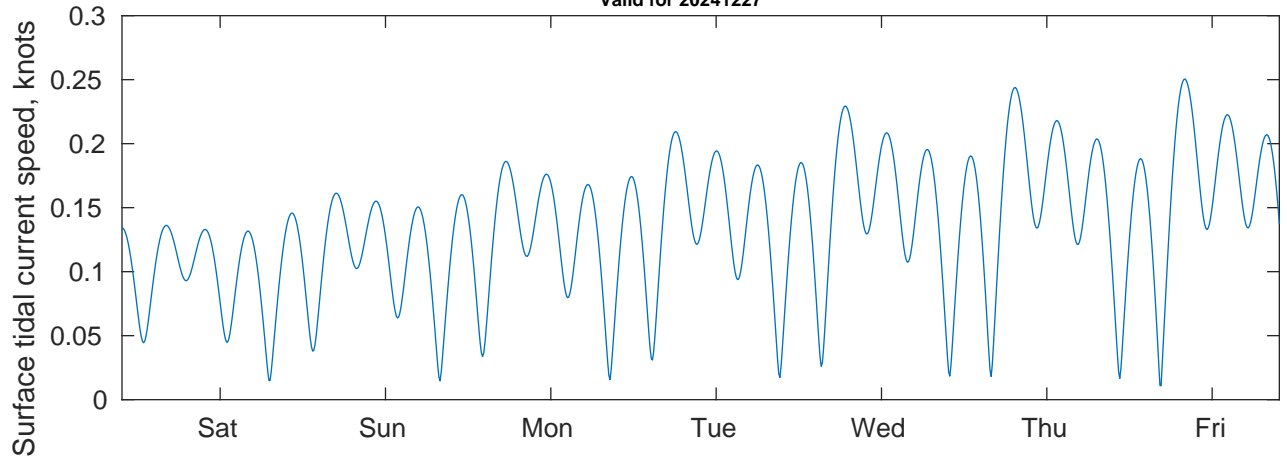
Tidal Currents and Heights for Nautilus at 20241227
