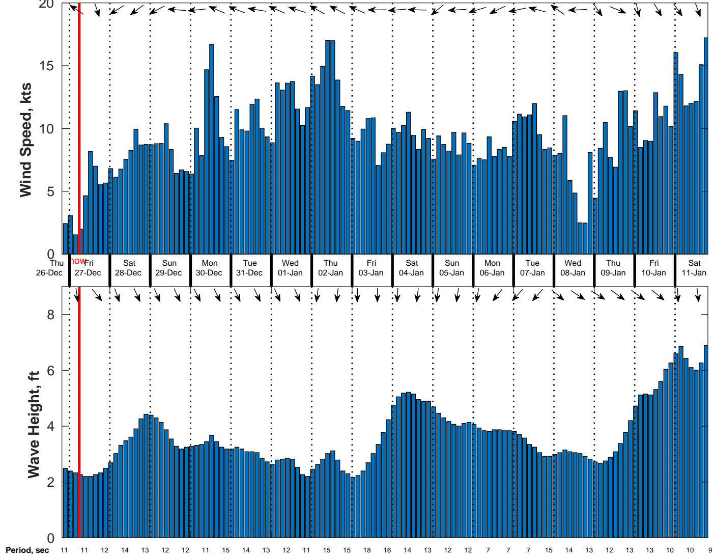
Wind & Wave Forecast for Nautilus from 26-Dec-2024 20:00:00 to 11-Jan-2025 20:00:00
