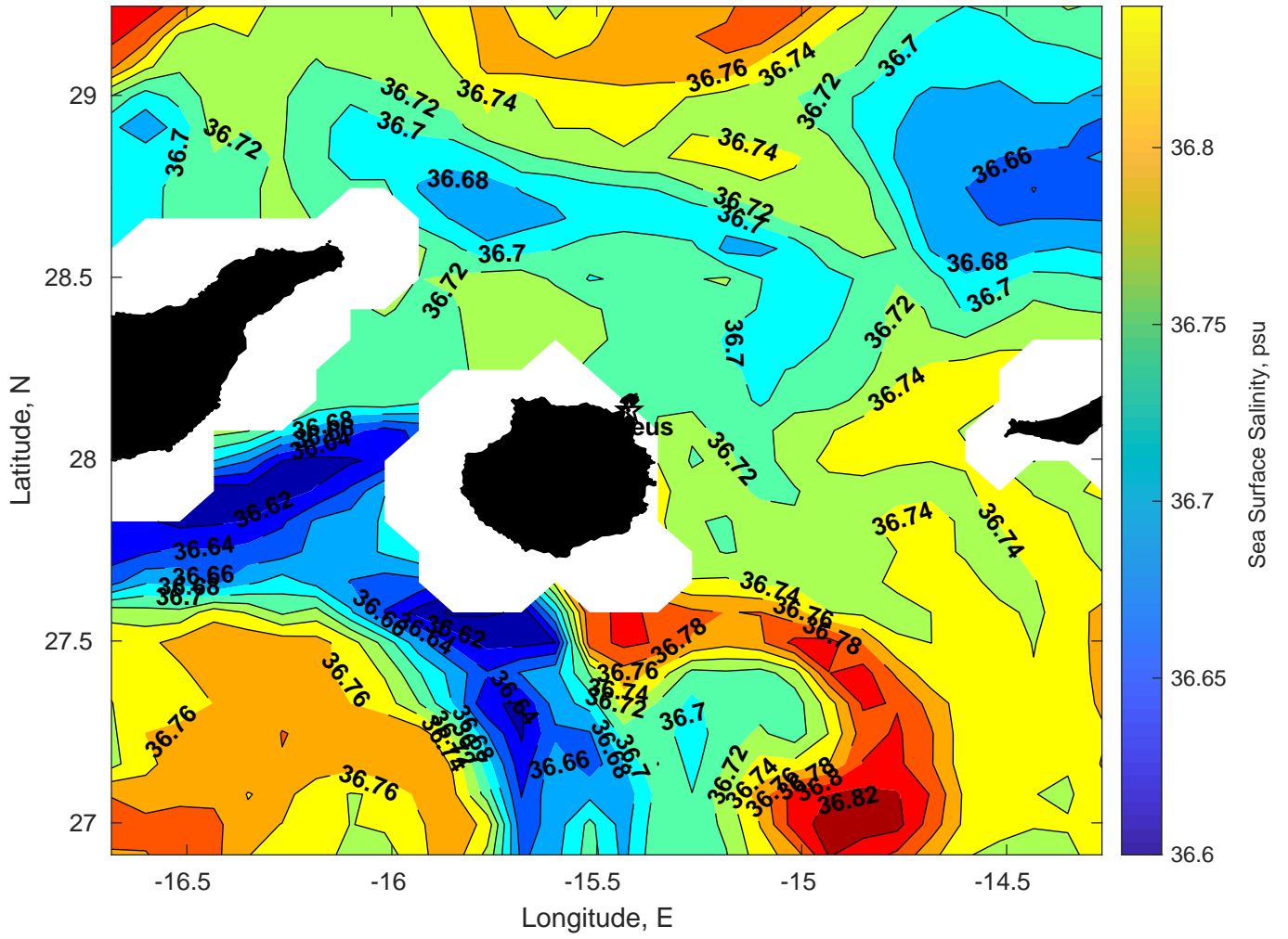
Surface Salinity for Proteus at 26-Dec-2024 00:00:00
