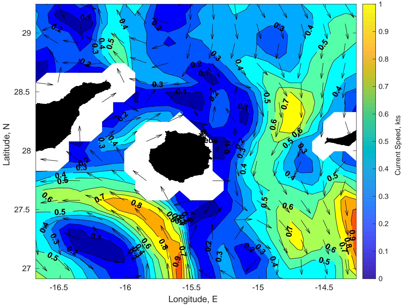
Surface Currents for Proteus at 26-Dec-2024 00:00:00
