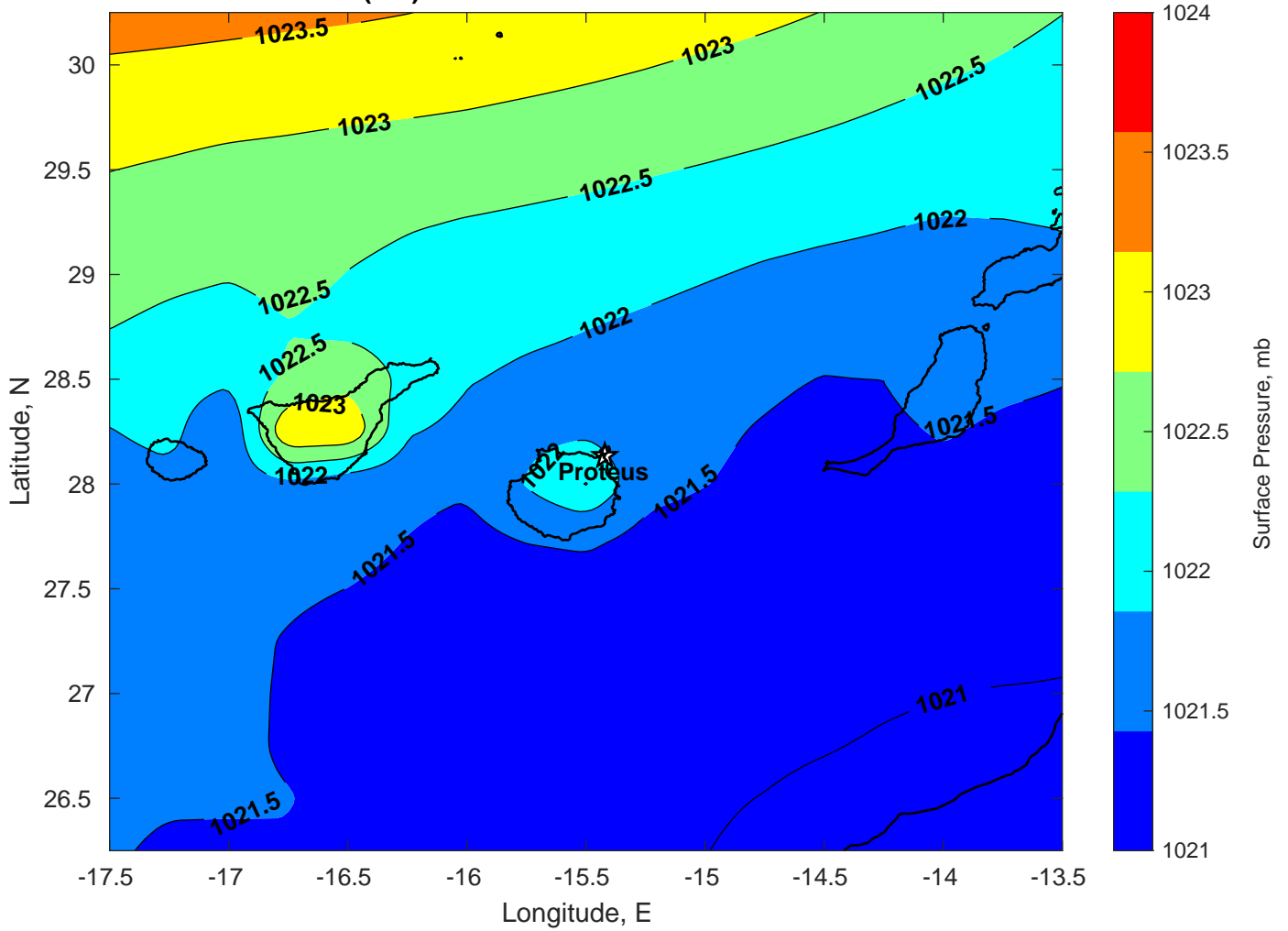
Surface Pressure (mb) for Proteus at 28-Dec-2024 00:00:00
